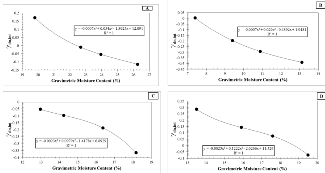
Figure 3.5: Plots of \gamma_{dn,int} versus moisture content for (A) Fayette County Clay, (B) Daviss County Clay, (C) Lee County Clay and (D) Warren County Clay.
