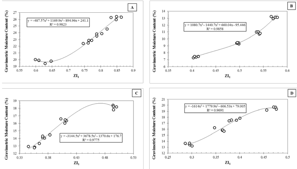
Figure 3.6: ZI_1 versus moisture content for (A) Fayette County Clay, (B) Daviss County Clay, (C) Lee County Clay and (D) Warren County Clay.
