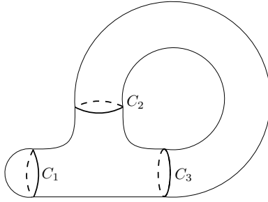
Figure 7.3: A simple DAP decomposition of a torus utilizing a disc enclosed by C_1 , an annulus enclosed by \{C_2, C_3\} and a pair of pants enclosed by \{C_1, C_2, C_3\} . This decomposition is not minimal in that the same manifold could have been decomposed using a single loop.
