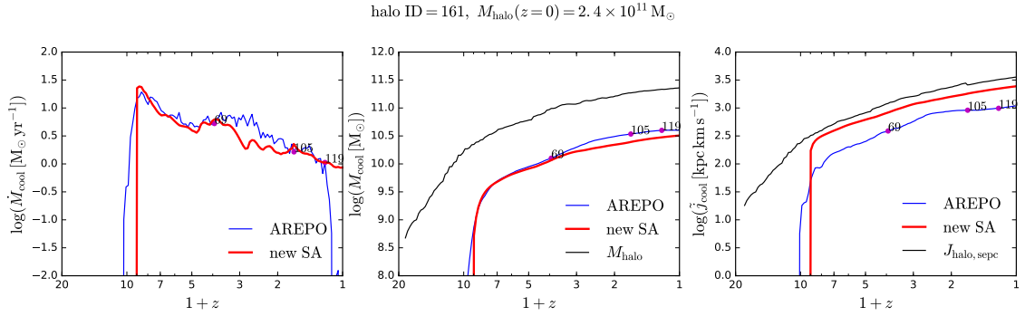
Figure 5.3: left : The predicted mass cooling rate. middle : The predicted cumulative cooled down mass. The growth of halo mass is also shown for reference. right : The predicted specific angular momentum \tilde{j}_{\text{cool}} of the cooled down gas. The evolution of the halo specific momentum is also shown as reference. In all three panels, the magenta points label the snapshots where further details are shown, and the associated numbers are the snapshot ids.
