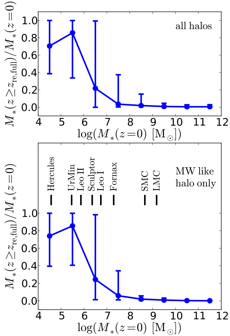
Figure 3.10: Fraction of stellar mass in galaxies at z = 0 which was formed before reionization (i.e. at z \geq z_{\text{re,full}} ). In both panels, each filled circle shows the median of the ratio in the corresponding z = 0 stellar mass bin, while the corresponding error bar indicates the 5 – 95% range of this ratio. Upper panel: All galaxies. Lower panel: Galaxies in Milky Way-like halos only (defined as halos with z = 0 halo mass in the range 5 \times 10^{11} M_\odot \leq M_{\text{halo}} \leq 2 \times 10^{12} M_\odot ). The short vertical solid black lines indicate the observed stellar masses of several Milky Way satellites, namely LMC, SMC, Fornax, Sculptor, Leo I, Leo II, Ursa Minor (UrMin) and Hercules, for reference (from McConnachie 2012 ).
