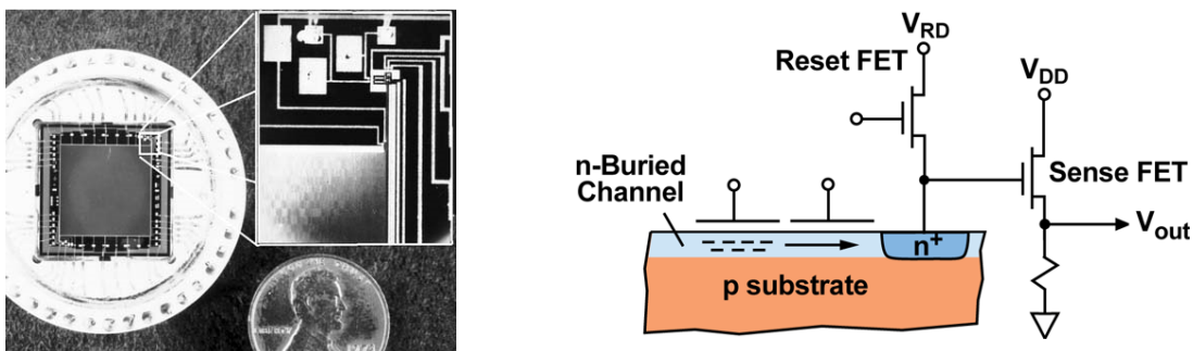
Fig. 4.11: Output amplifier imprinted at the corner of a CCD (left image) and equivalent electronic circuit (right image), composed of FET transistors. Images courtesy Texas Instruments and Lincoln Laboratories.
