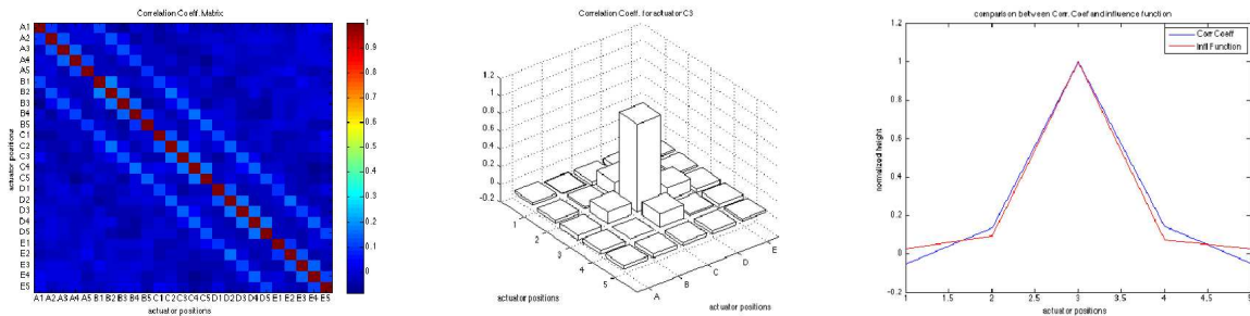
Fig. 3.7: Left panel: correlation coefficients matrix R ; central panel: correlation coefficients for the central actuator, taken from matrix R ; right panel: comparison between a traditional influence function and the correlation coefficients.
