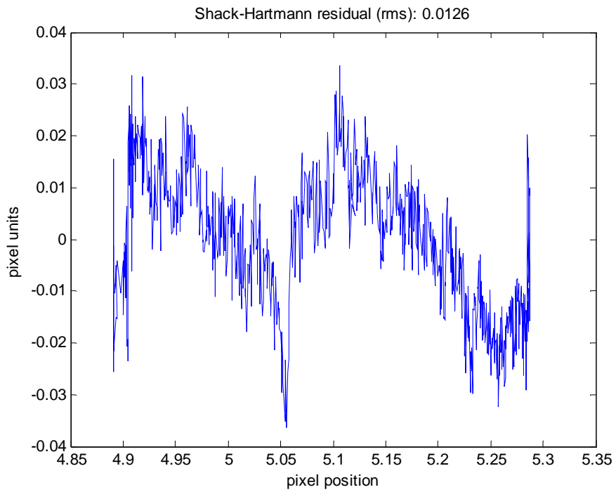
Fig. 4.36: SH residual error (value in the title of the plot) after calibration for ADC = 8 bits.
