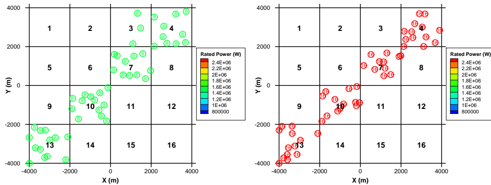
(b) The optimal solution with the minimum COE ( COE = 0.0361\$/kWh , A_{MW} = 43.39ha/MW ) (c) The optimal solution with the minimum COE ( COE = 0.0432\$/kWh , A_{MW} = 15.67ha/MW )
