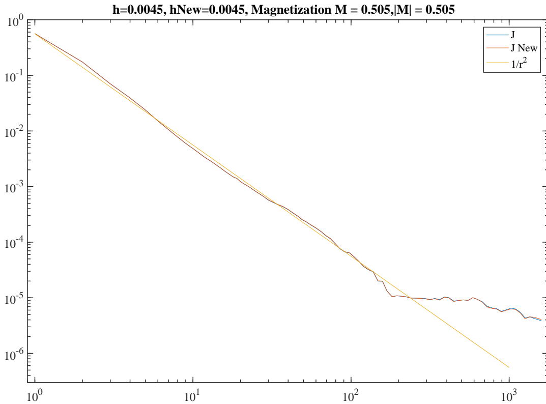
Figure 4.9: Profile of long-range interaction for Maxima Entropy Model
