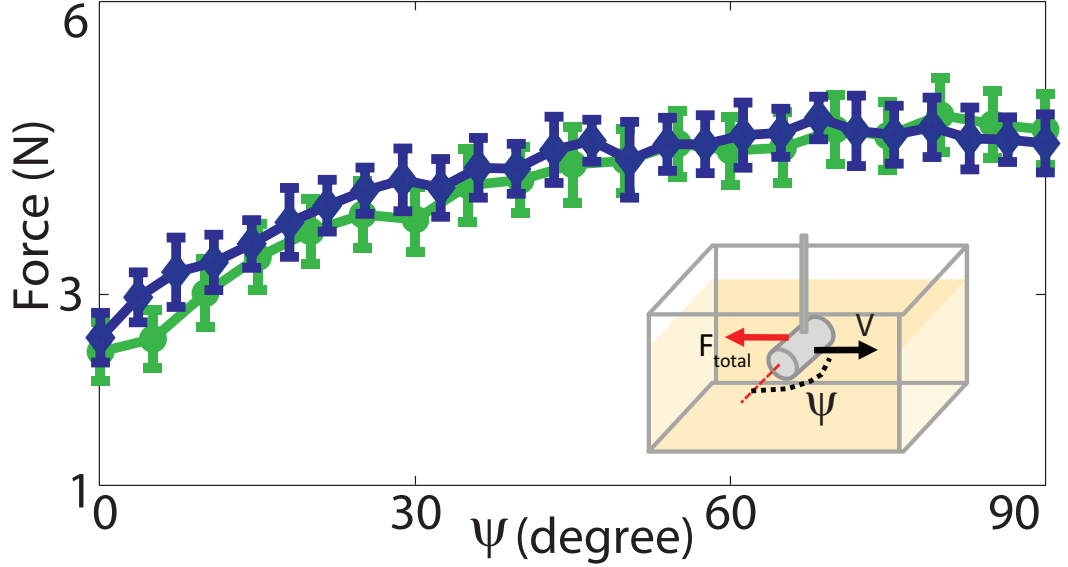
Figure 36: Simulated granular media was validated by comparing the forces on a rod dragged through it with those measured from experiment. Total force on a stainless steel rod (sides and ends) (diameter = 15.8 mm, length = 40 mm, and rod-particle static friction coefficient \mu_{bp} = 0.15 ) immersed to a depth of 7.62 cm was measured as a function of the angle ( \psi ) between the velocity direction and its orientation in experiment (green) and simulation (blue) in a loosely packed medium. The inset shows the experimental setup.
