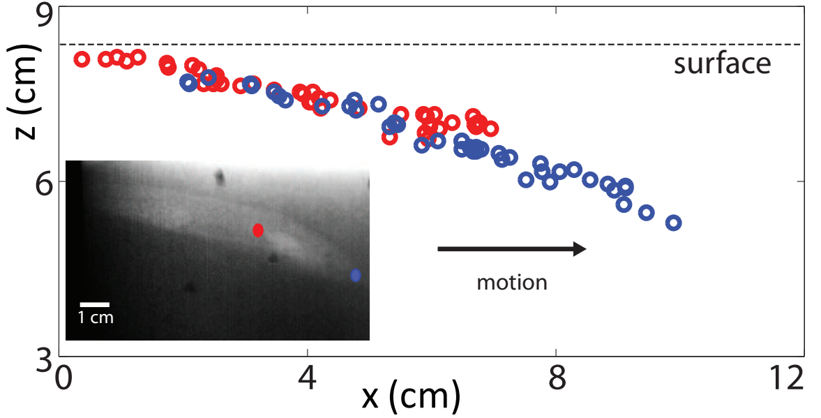
Figure 31: Sagittal plane view of the sandfish trajectory as it swam subsurface obtained using x-ray imaging. The blue and red circles correspond to the position of the animal’s snout and 40% of its body-length measured from its snout. Inset shows a side view x-ray image of the sandfish as it swam within 0.3 mm glass particles.
