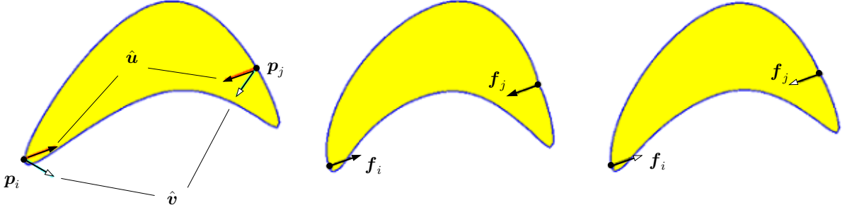
Figure 3.2 Comparison between unit stable and pure squeezes.
