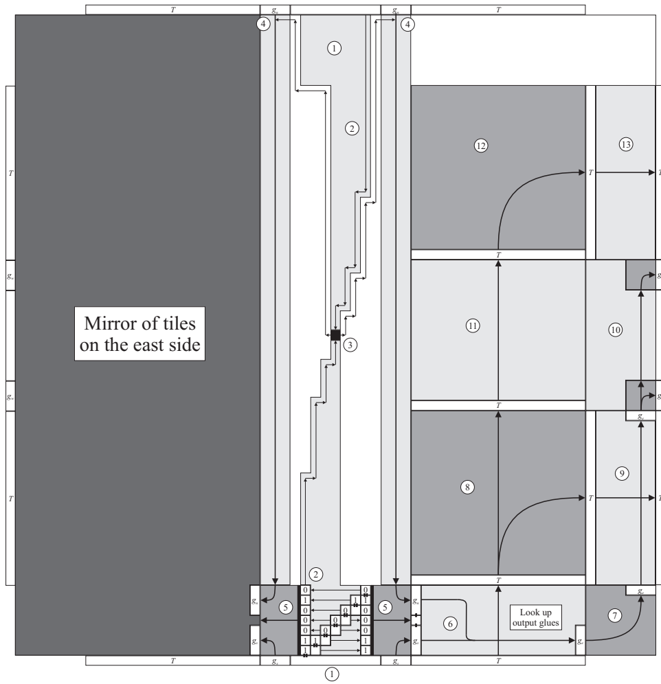
Figure 5.1: NS supertile
