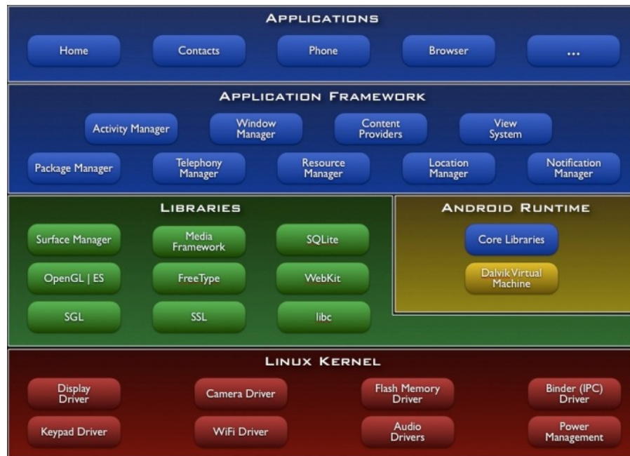
Figure 5 Android architecture [24]
