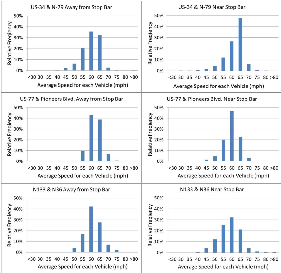
Figure D-1 Speed Distribution for 0 mph Speed Reduction Group
