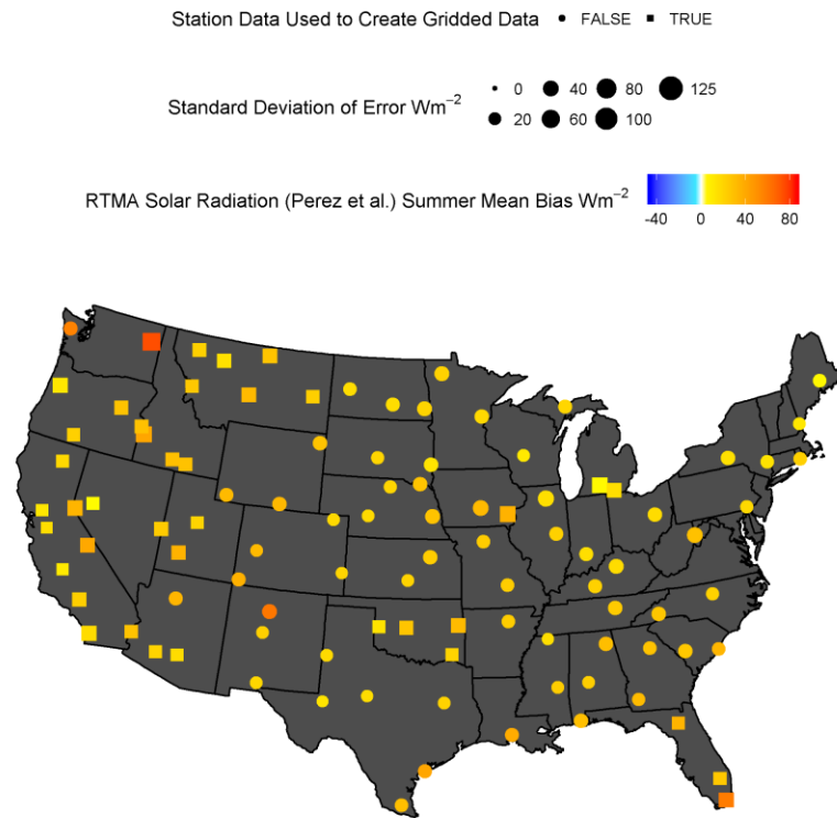
Figure 8.6 RTMA shortwave solar radiation estimated using the Perez et al. method mean bias and standard deviation of error computed using summertime daily data for 2015.
