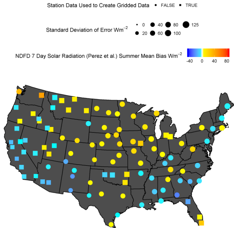
Figure 8.7 NDFD day 7 shortwave solar radiation estimated using the Perez et al. method mean bias and standard deviation of error computed using summertime daily data pooled across all study years.
