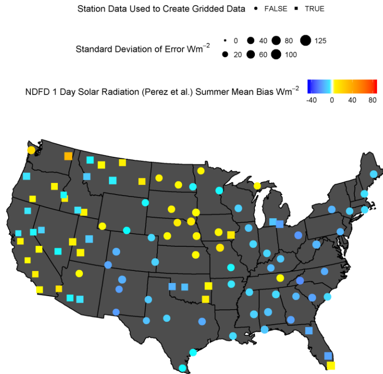
Figure 8.8 NDFD day 1 shortwave solar radiation estimated using the Perez et al. method mean bias and standard deviation of error computed using summertime daily data pooled across all study years.
