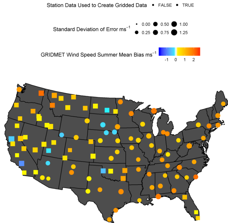
Figure 8.13 GRIDMET wind speed mean bias and standard deviation of error computed using summertime daily data pooled across all study years.
