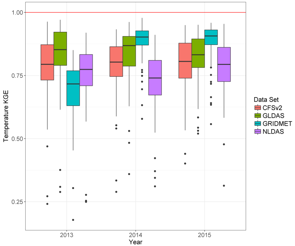
Figure 5.5 Near-surface air temperature KGE computed for the summer of each study year.
