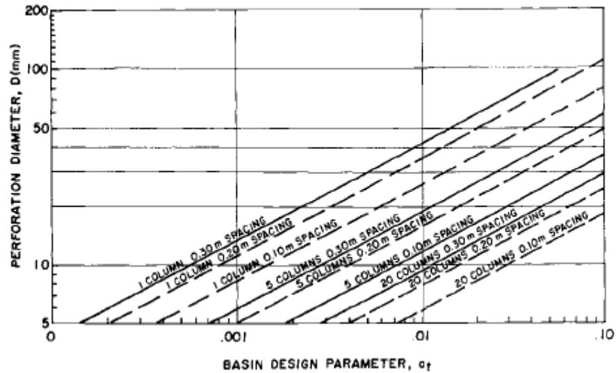
Figure 2-3 Perforated Riser Design Space (Jarrett 1993)
