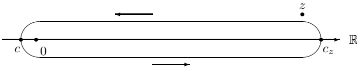
Figure 3.7: Contour (c, c_z)
