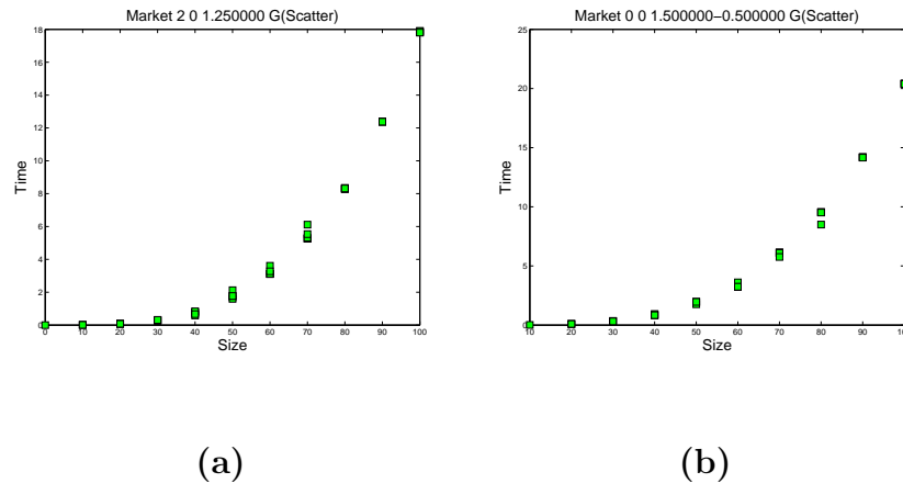
Figure 4.4: The running time of PATH, in seconds, as a function of the input size ( m = n ). (a) The concentrated generator is used for the desirability matrix and the uniform generator for the endowment matrix; \sigma_t = \sigma_b = 1.25 . (b) The uniform generator is used for both the desirability and endowment matrix; \sigma_t = 1.5 and \sigma_b = 0.5 . There were five runs for each input size.
