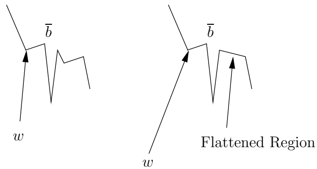
Figure 2.13: The left picture shows what the b variable gadget originally looked like in C_{i-1} in Figure 2.12. The right picture shows the modified variable gadget to contain the clause distinguished point.
