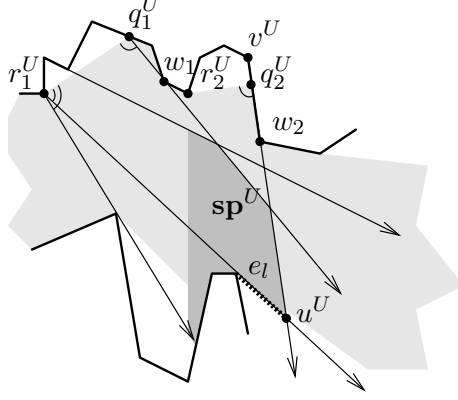
Figure 5.8: Computing the upper spear and the base.
