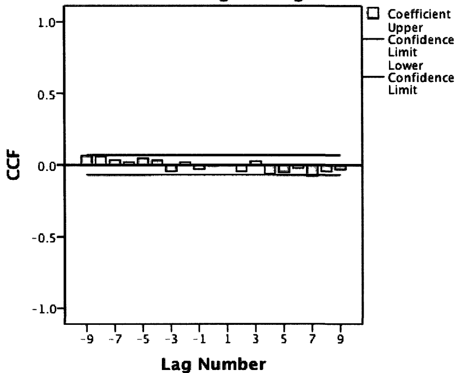
Figure 9 Cross-Correlation Function of blood glucose and Vmag for subject 84
