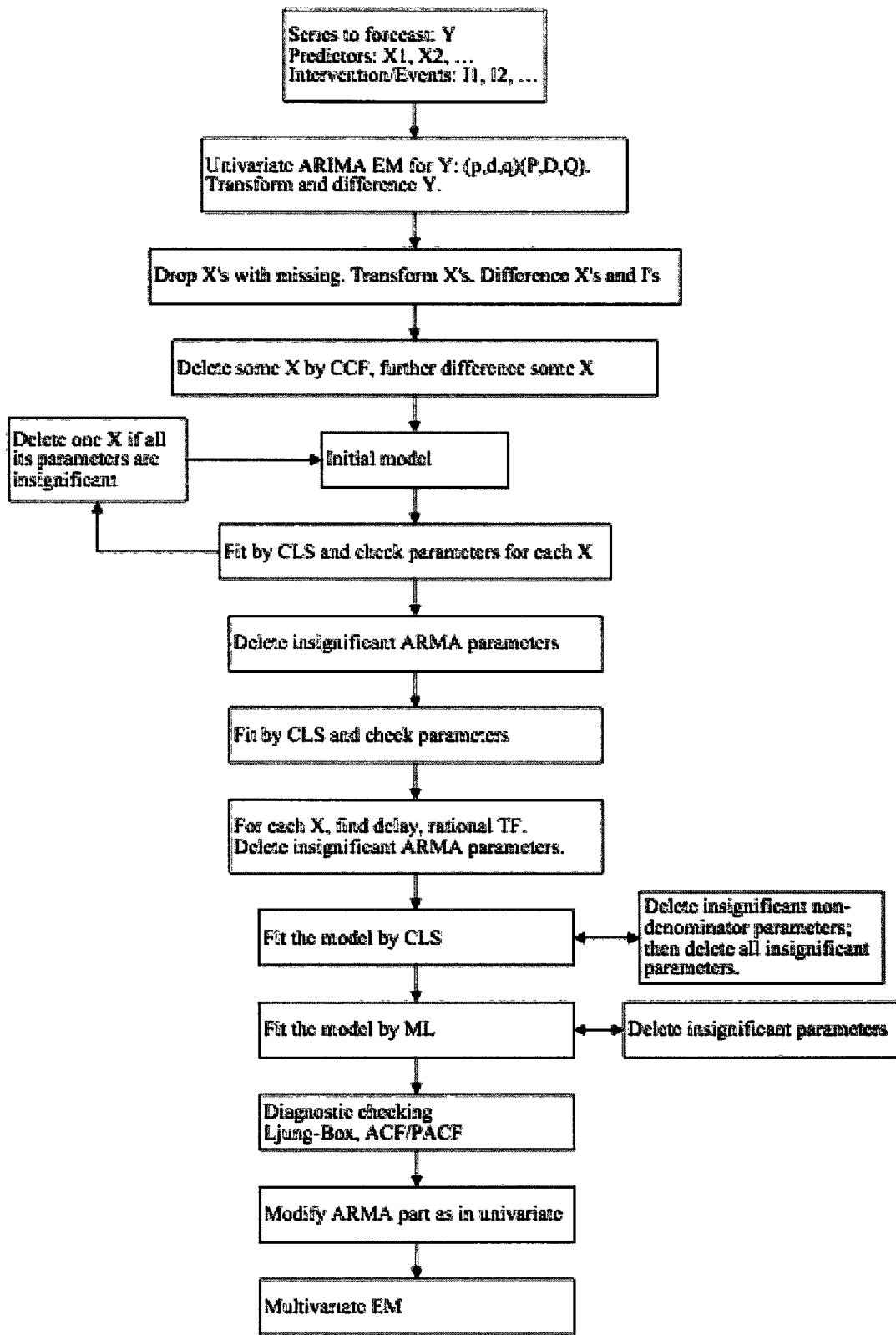
Figure 7 Software time series algorithm model concept (SPSS, 2004)
