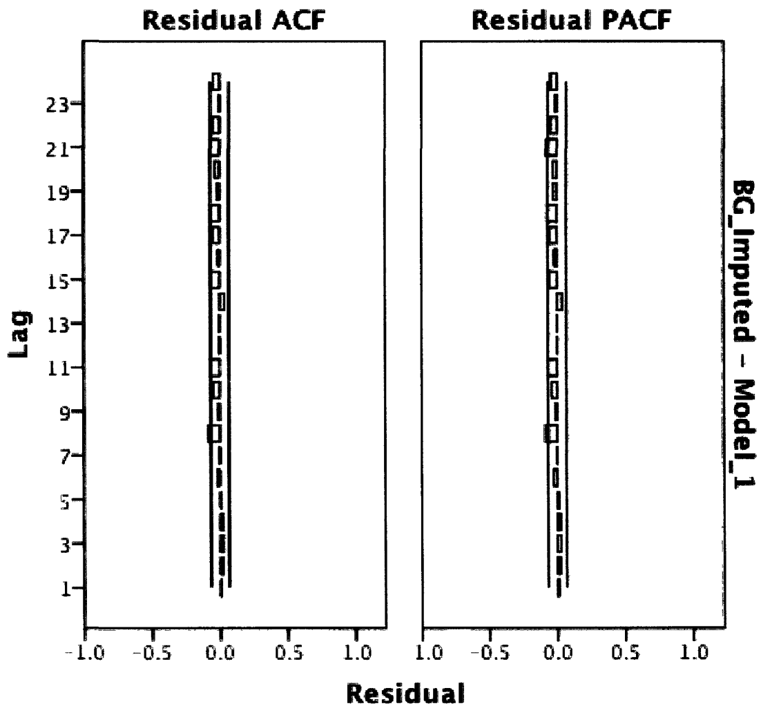
Figure 8 ACF and PACF residual plots for subject 84
