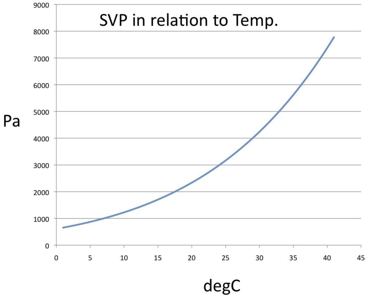
Figure 3: SVP in relation to Temperature (°C) (Murray 1967)
