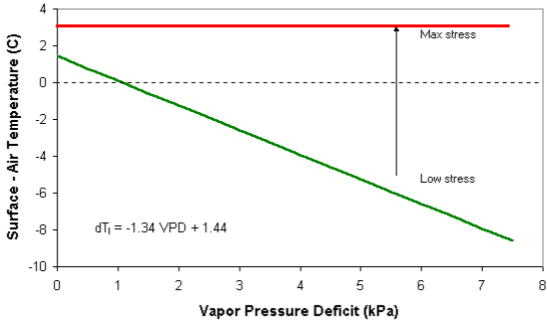
Figure 4: VPD baseline example (Idso et al, 1981)
