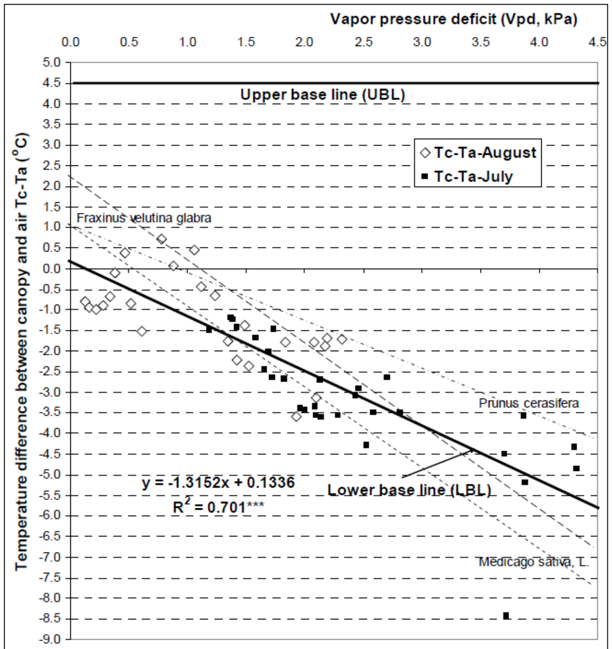
Figure 7: Chi and Growing's (2007) VPD baseline for apple
