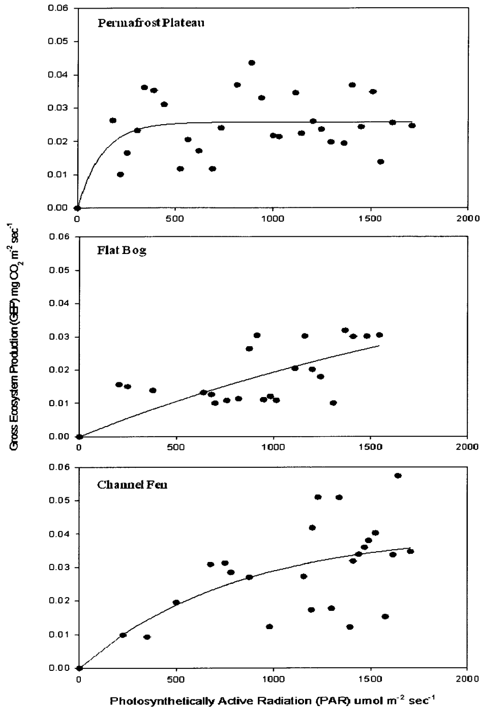
Figure 5-2 Relationship between gross ecosystem production (GEP) of CO 2 and photosynthetically active radiation (PAR) for 2008 at Scotty Creek, Northwest Territories, Canada. Showing the variation between landscape units: permafrost plateau (n=104, r 2 =0.3), flat bog (n=110, r 2 =0.4), and channel fen (n=84, r 2 =0.4). The fitted curve for GEP versus PAR is an exponential model from Eq. (3.7). Symbols denote GEP bin-averages based on PAR intervals of 10 μmol m -2 sec -1 .
