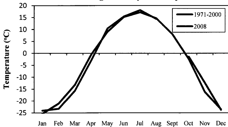
Figure 2-3 Fort Simpson climate normals for 1971-2000 and monthly averages for 2008 (Data Source: Environment Canada, 2010).
