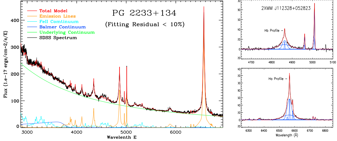
Fig-2a: An Example of SDSS Spectrum Fitting
