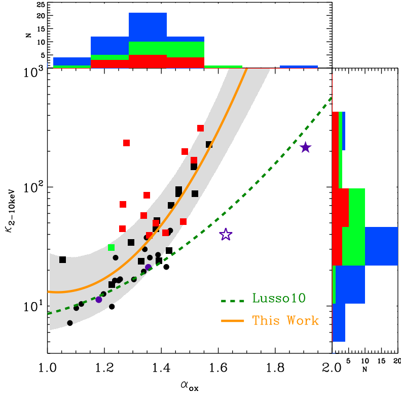
Figure 5.4: \kappa_{2-10\text{keV}} vs. \alpha_{ox} . Each symbol represents the same type of source as in Figure 5.2. The solid orange line is the best fit line found using a second order polynomial, and the shaded area is the \pm 1\sigma zone.
