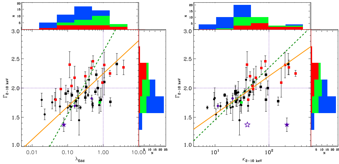
Figure 5.8: \Gamma_{2-10\text{keV}} vs. \lambda_{Eddr} and \kappa_{2-10\text{keV}} . Each symbol represents the same type of source as in Figure 5.2. In the left panel, the solid orange line is the bisector regression line. The dashed green line is that reported by Zhou10b. The vertical and horizontal purple lines are for \Gamma_{2-10\text{keV}}=2 and \lambda_{Eddr}=1 . The symbols and lines in the right panel have the same meaning as those in the left panel. The vertical purple line is for \kappa_{2-10\text{keV}}=100 . PG 1004+130 was excluded when performing the regression, but assuming its intrinsic X-ray flux to be 1 dex higher and a \Gamma_{2-10\text{keV}} \sim 1.8 would make it consistent with the other sources. It is shown as the open purple star in both panels.
