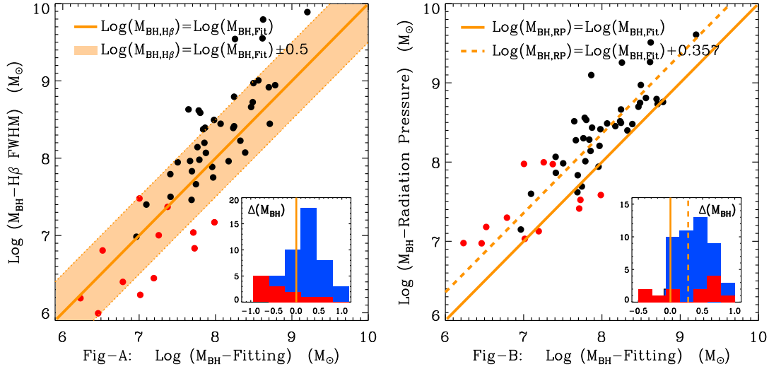
Figure 3.11: Correlations of best-fit black hole mass ( M_{BH-Fitting} or M_{BH,FIT} ) vs. H\beta FWHM determined black hole mass ( M_{BH-H\beta} \text{ FWHM} or M_{BH,IC+BC} ) and vs. radiation pressure corrected black hole mass ( M_{BH-Radiation Pressure} or M_{BH,RP} ). Red points represent the 12 NLS1s. The inserted panel in panel-A shows the distribution of the mass difference between M_{BH,IC+BC} and M_{BH,FIT} , while the inserted panel in panel-B shows the distribution of the mass difference between M_{BH,RP} and M_{BH,FIT} . Red regions highlight the distribution of NLS1s.
