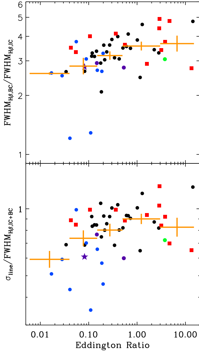
Figure 4.10: The H\beta line shape correlation with Eddington ratio. The upper panel uses \text{FWHM}_{BC}/\text{FWHM}_{IC} to represent H\beta shape, while the lower panel uses \sigma_{line}/\text{FWHM}_{IC+BC} instead. In each panel the various symbols represent the same type of sources as in Figure 4.3. The orange data points are the binned data for different Eddington ratio bins with 1 standard error on the Y-axis.
