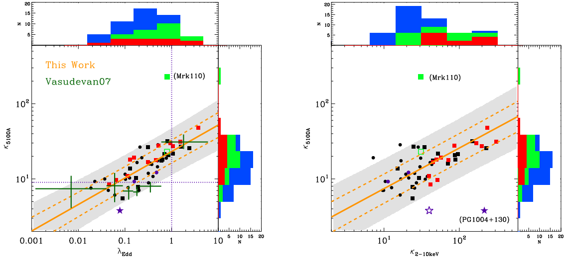
Figure 5.7: \kappa_{5100} vs. \lambda_{Edd} and \kappa_{2-10keV} . Each symbol represent the same type of source as in Figure 5.2. In the left panel, the solid orange line is the OLS line assuming \lambda_{Edd} to be the independent variable. The two dashed orange lines show the \pm 1\sigma region, and the shaded region is the \pm 2\sigma region. The green open square symbol is Mrk 110 reported by Landt et al. (2011). The vertical and horizontal purple lines are for \kappa_{5100}=9 and \lambda_{Edd}=1 . The symbols and lines in the right panel have the same meaning as those in the left panel.
