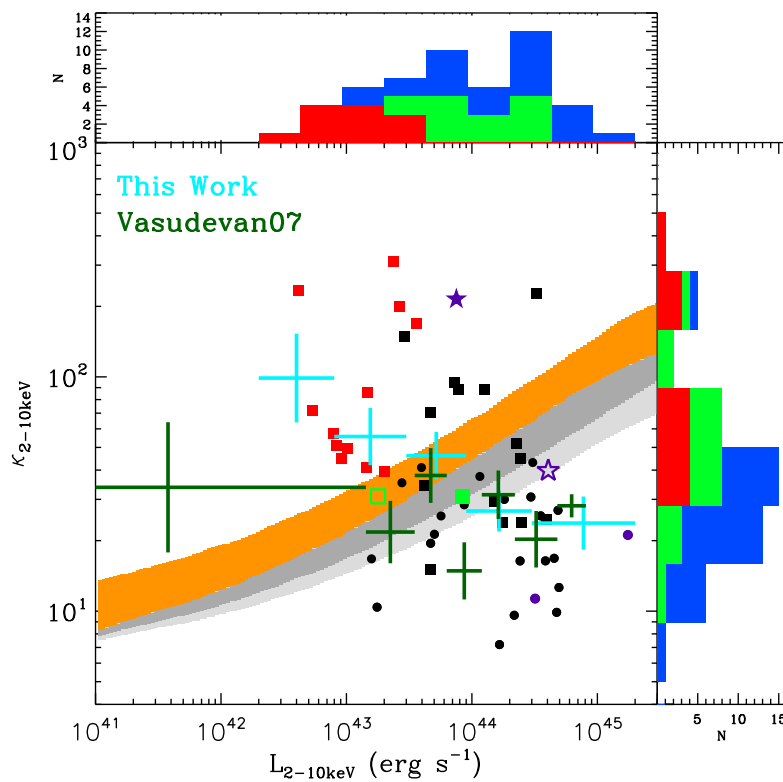
Figure 5.11: \kappa_{2-10keV} vs. L_{2-10keV} . Different symbols represent the same type of sources as in Figure 5.2. The orange and gray shaded regions represent the theoretical \kappa_{2-10keV} with \pm 1\sigma scattering at each L_{2-10keV} in Hopkins07 and Marconi04. The green data points are reproduced from Fig.3 in VF07.
