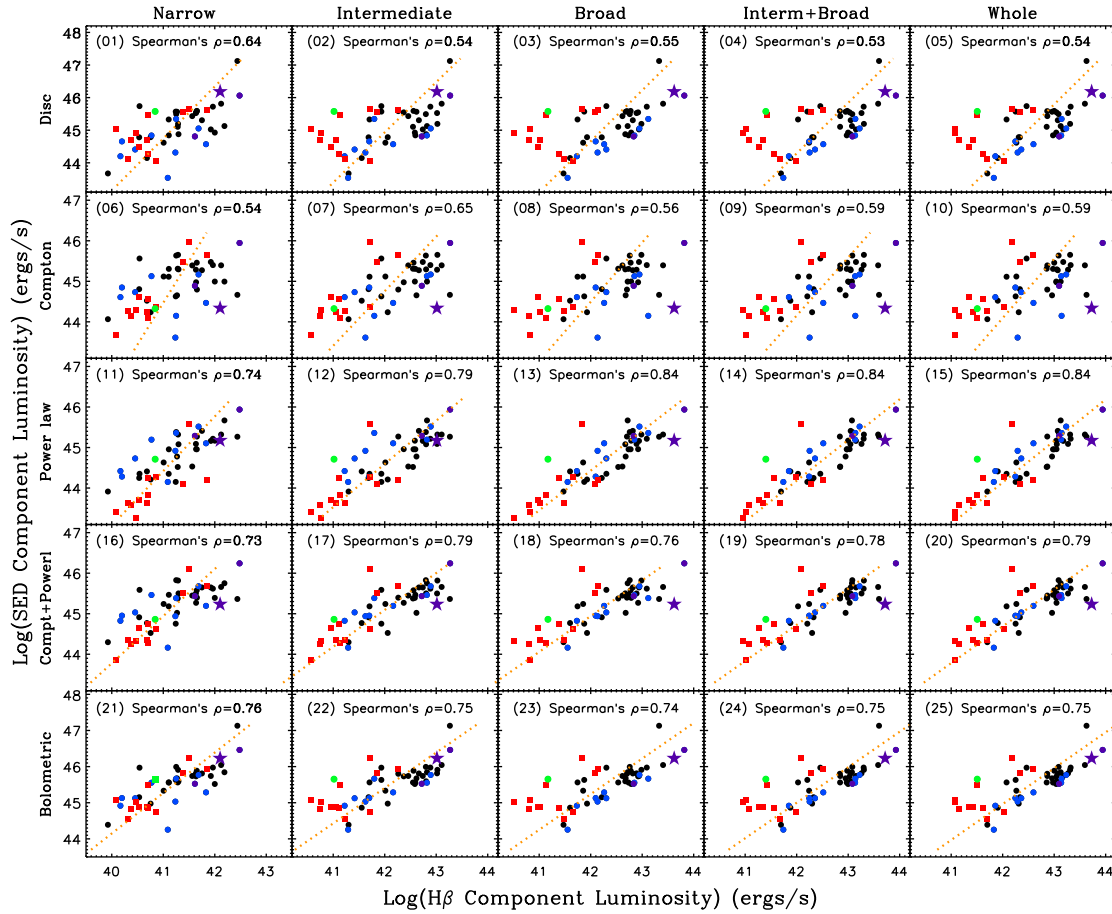
Figure C.1: The luminosity correlations between H\beta line components and SED components. Red points represent NLS1s; blue points represent the broadest H\beta line BLS1s; green point is Mrk 110; purple star is PG 1004+130; purple symbols indicate radio loud sources. The orange dotted line denotes the OLS regression line assuming the SED component luminosity is the independent variable. Spearman's rank correction coefficient \rho_s for the whole sample is also given in each panel.
