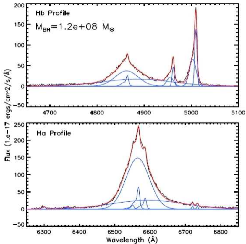
Figure 1.11: An example of broad H \alpha and H \beta emission lines, along with nearby emission lines such as [OIII] \lambda\lambda 4959,5007, [NII] \lambda\lambda 6548,6584 and [SII] \lambda\lambda 6716,6731, from the SDSS spectrum of RBS 1423, fitted with multiple Gaussian components (blue solid lines). The red solid line is the sum of all the Gaussian components. This figure is reproduced from Jin et al. (2011).
