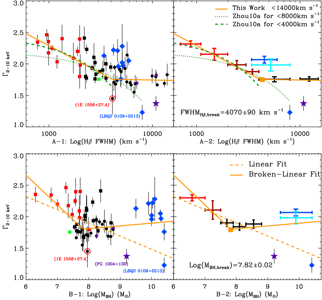
Figure 5.9: \Gamma_{2-10 \text{ keV}} vs. FWHM of \text{H}\beta and M_{\text{BH}} . In the upper left panel, a broken line is fitted to the sample using the minimum \chi^2 method. S06,08 proposed the linear correlation between \Gamma_{2-10 \text{ keV}} and \text{Log}(\text{H}\beta \text{ FWHM}) was not followed by their 10 extremely high luminosity sources, so we plot their sample as blue diamond symbols for comparison. In the right panel binned points are plotted with 1 standard error of \Gamma_{2-10 \text{ keV}} in order to show the break points more clearly. The two red points only include the NLS1s, the two dark points are the broadest BLS1s. The cyan point is the binned point for the whole sample of S06,08. The blue point is the binned point for S06,08's sample but excluding LBQS 0109+0213 whose \Gamma_{2-10 \text{ keV}} is anomalously low. The square orange point is the break point. 1E 1556+27.4 shown by the red circle is another source with \Gamma_{2-10 \text{ keV}} < 1.5 . In the second row, the symbols all have the sample meaning as in the first row. We plot the linear regression line as the dashed orange line.
