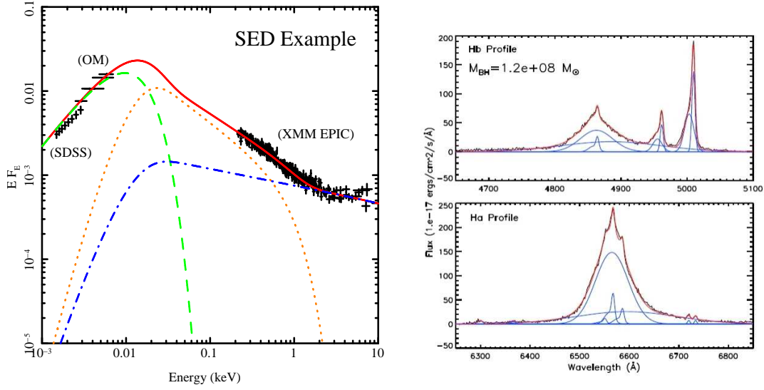
Figure 4.1: Examples of spectral fitting in Chapter 3. Left panel shows the broadband SED fitting of PG 1115+407 which consists of a modified accretion disc (green dashed line), a soft X-ray Comptonisation (orange dotted line) for the soft X-ray excess and a hard X-ray Comptonisation (blue dash-dotted line) for the hard X-ray power law tail. Right panel shows the emission line fittings of RBS 1423 around H\alpha and H\beta . Blue solid lines represent different line components.
