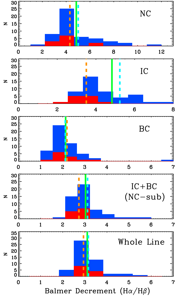
Figure 4.8: Balmer decrement distributions of different Balmer line components. In each panel the entire histogram shows the distribution of the whole sample, with green solid line indicating the mean decrement value. Red region highlights the distribution of the 12 NLS1s and the orange dashed line indicates their mean decrement value. The cyan dashed line shows the mean decrement value of the BLS1s. The mean decrements are also listed in Table 4.2.
