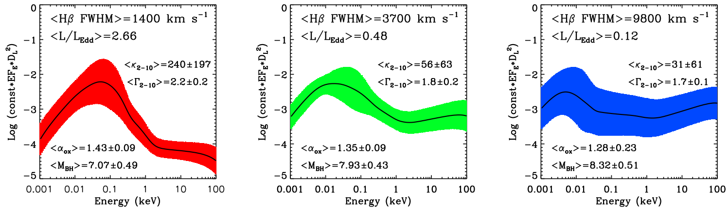
Figure 3.12: The average SED of our sample. The panel on the left shows the averaged SED for the 12 NLS1s (including two marginal NLS1s, 2XMM 112328.0+052823 and 1E 1346+26.7). The average H\beta FWHM is 1400 \pm 500 \text{ km s}^{-1} . The red area indicates a one standard deviation region on either side of the average spectrum. The central panel is for 12 objects with moderate line width. The average FWHM is 3700 \pm 600 \text{ km s}^{-1} . The green region indicates one standard deviation. The panel on the right is the mean SED for the 12 broadest line objects in our sample, including the one double-peak source. The average FWHM is 9800 \pm 2900 \text{ km s}^{-1} . We also show the average value of the 2-10 keV power-law photon index, the 2-10 keV bolometric correction, and the \alpha_{\text{ox}} value with a one sigma error. D_L on the Y-axis title is the luminosity distance. The unit of Y-axis is ‘keV (ergs \text{s}^{-1} \text{ keV}^{-1} )’ in logarithm. The same arbitrary constant of 1.31 \times 10^{-46} is used for rescaling each plot.
