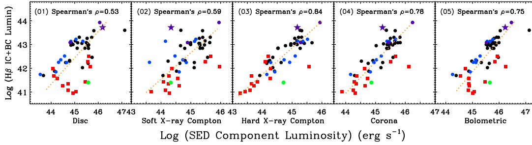
Figure 4.4: The luminosity correlations between H\beta IC+BC and broadband SED components. ‘Corona’ means the coronal luminosity, which is the sum of the luminosities of the soft and hard X-ray Comptonisation components. Different symbols represent different type of sources as explained in Figure 4.3. In each panel the Spearman’s rank coefficient is given, along with the orange dotted line indicating the bisector regression line.
