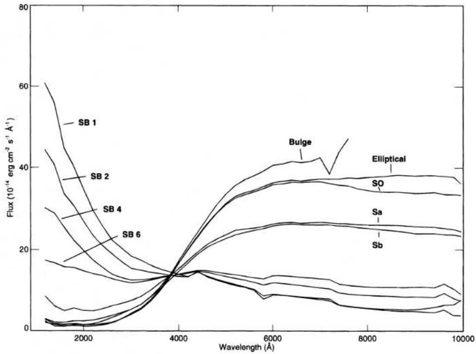
Figure 1.10: Spectral templates (binned in 200\text{\AA} ) for different types of host galaxies, normalised at 4000\text{\AA} . ‘SB’ represents starburst galaxy template with different E(B-V) : SB 1 for E(B-V) \leq 0.10 ; SB 2 for 0.11 \leq E(B-V) \leq 0.21 ; SB 4 for 0.39 \leq E(B-V) \leq 0.50 ; SB 6 for 0.61 \leq E(B-V) \leq 0.70 . Figure is taken from Kinney et al. (1996).
