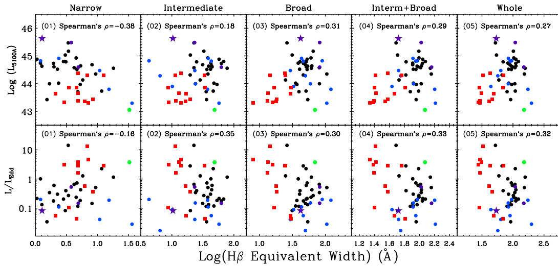
Figure C.2: The cross-correlation plots between \text{H}\beta line component EWs and L_{5100\text{\AA}} (the monochromatic luminosity at 5100\text{\AA} ) and L/L_{Edd} (the Eddington ratio). Different symbols have the same meaning as in Figure C.1. Spearman's \rho is given in each panel.
