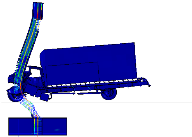
a) 120 km/h impact velocity
