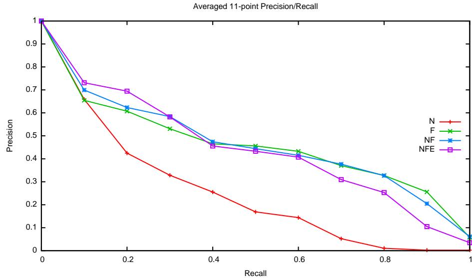
Figure 7.1. Averaged 11-point precision recall curve for surface pattern relations
