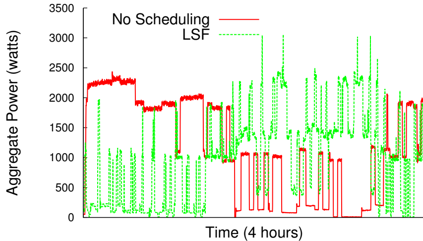
Figure 3.10. Power usage with and without LSF scheduling using using our smart home testbed with real background loads over a 4-hour period.
