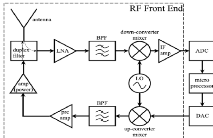
Figure(3.1):Transceiver system
