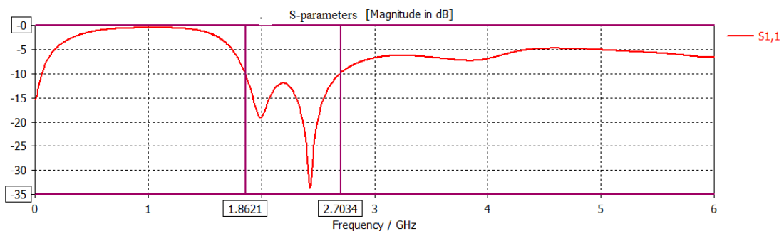
Figure(4.6): Simulated return loss ( S_{11} ) with ( W_2=45\text{mm} )
