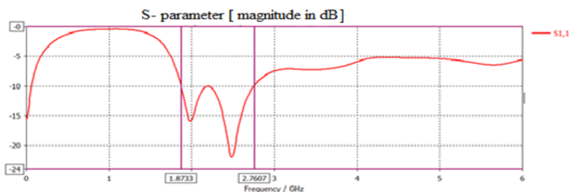
Figure(4.4): Simulated return loss ( S_{11} ) with (W2=55mm)
