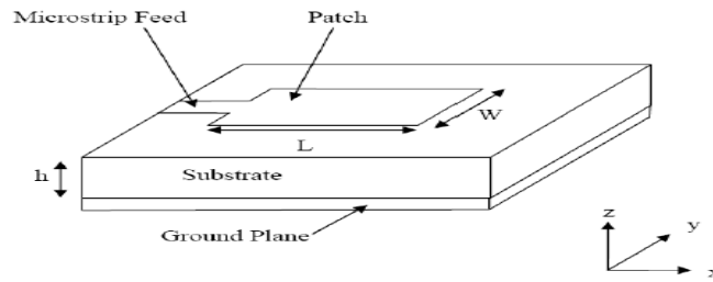
Figure(2.18): Microstrip patch antenna.( Girase, Tiwari, Sharma, Singh , 2014)
