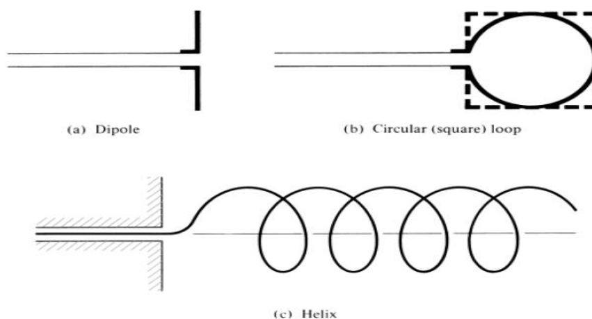
Figure (2.2): Wire antenna configurations
