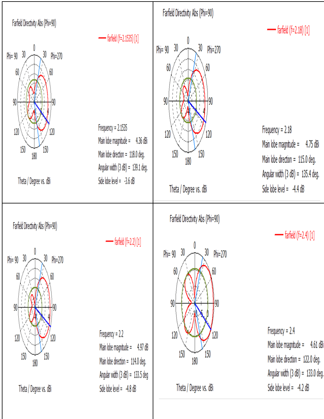
Figure(4.14): Simulated radiation patterns and the gains at different frequencies for modified antenna with large right triangle(W1=45mm).
