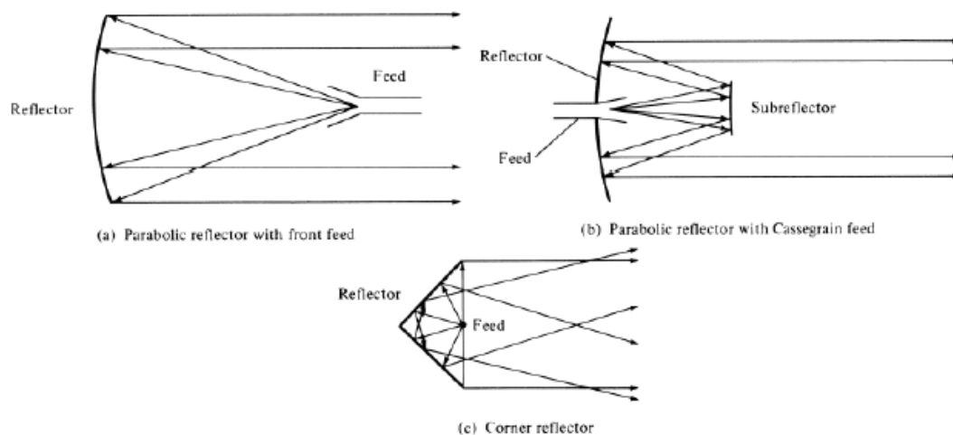
Figure(2.6): Typical reflector configurations. (Balanis, 2005)
