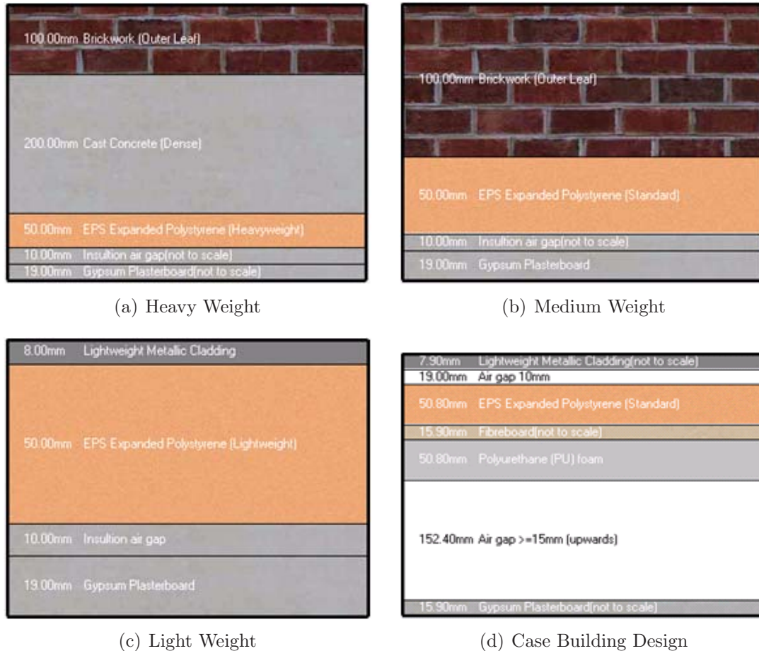
Figure 6.11: Case Building Envelope Design Prototypes
