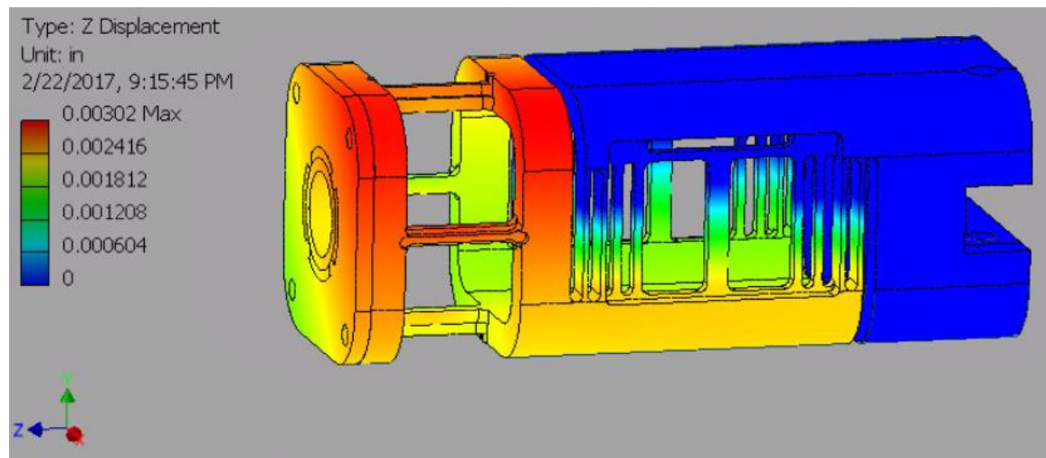
Figure 43: Z-Displacement
