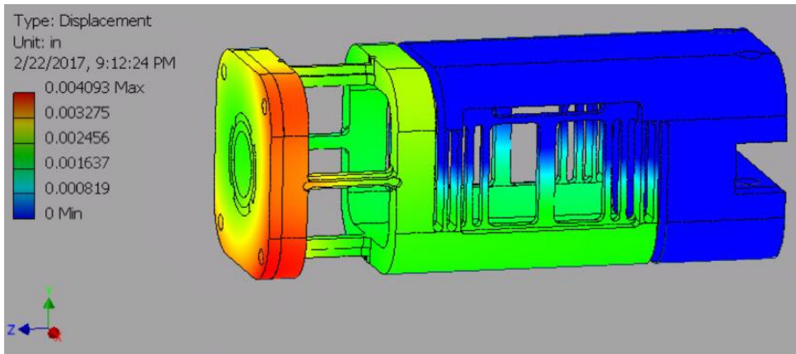
Figure 42: Resultant Displacement
