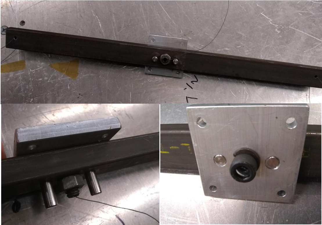
Figure 29: Calibration Adapter
