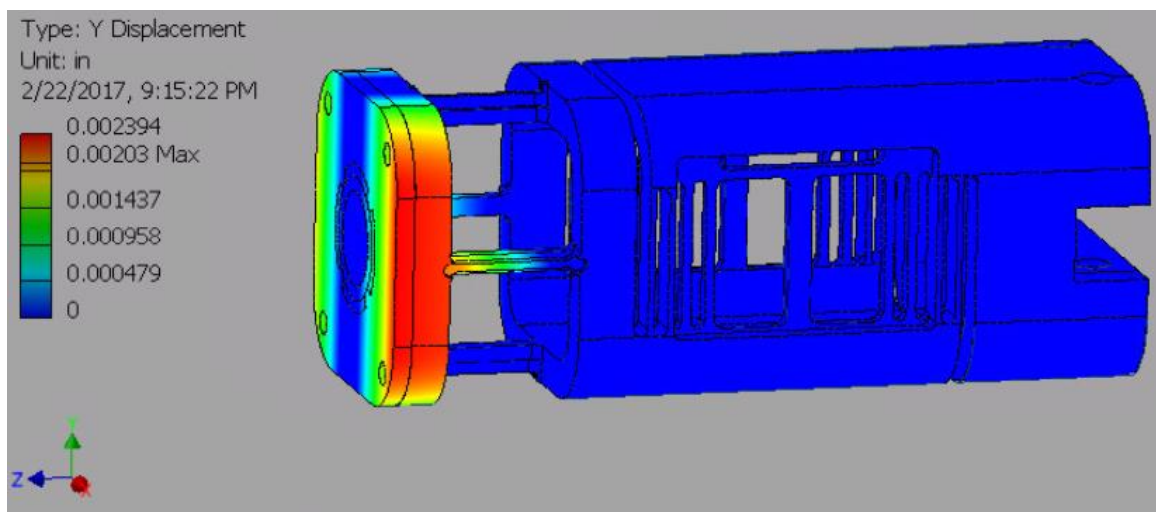
Figure 44: Y-Displacement
