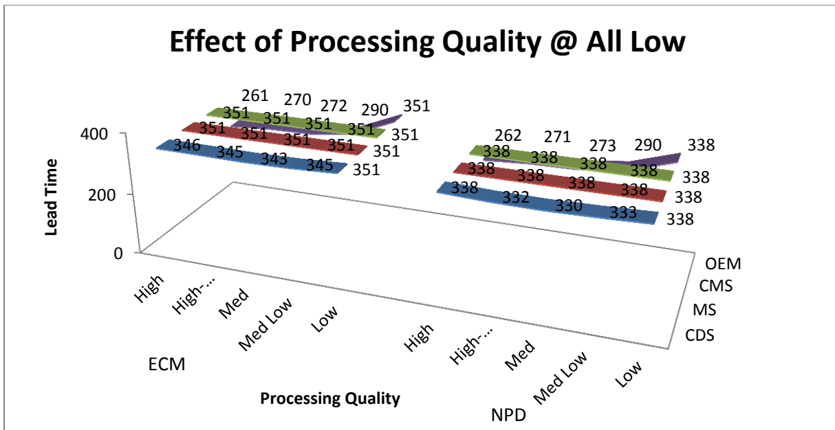
Figure 56: Effect of Processing quality on lead time when all variable are set constant at low
