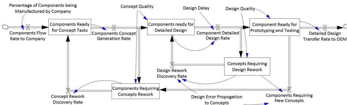
Figure 27: The Model Template for Supplier involved in Concept and Design phases
