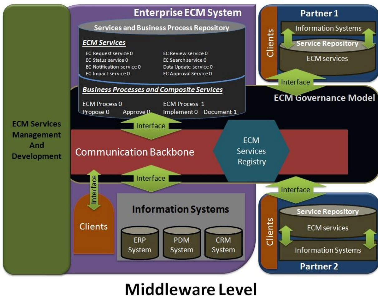
Figure 16: Middleware level components of the proposed SOA based ECM system
