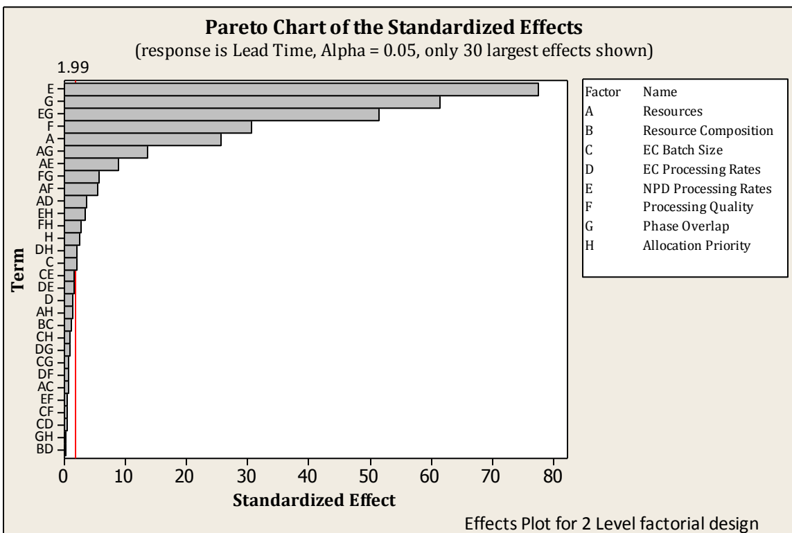
Figure 40: Effects of process parameters and their interactions on the NPD lead time.
