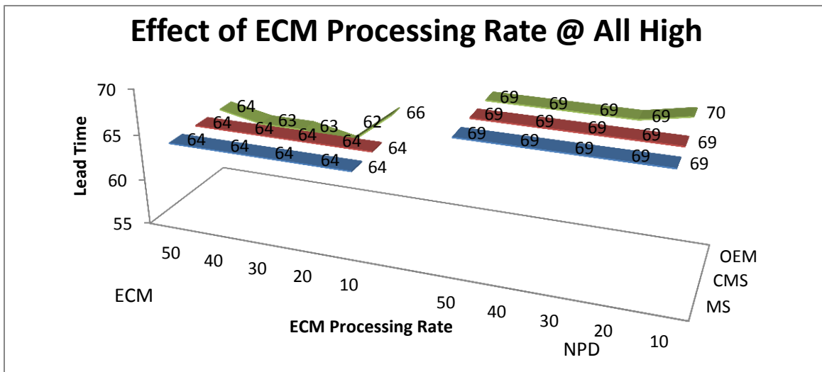
Figure 59: Effect of ECM Processing rate on lead time when all variable are set constant at high
