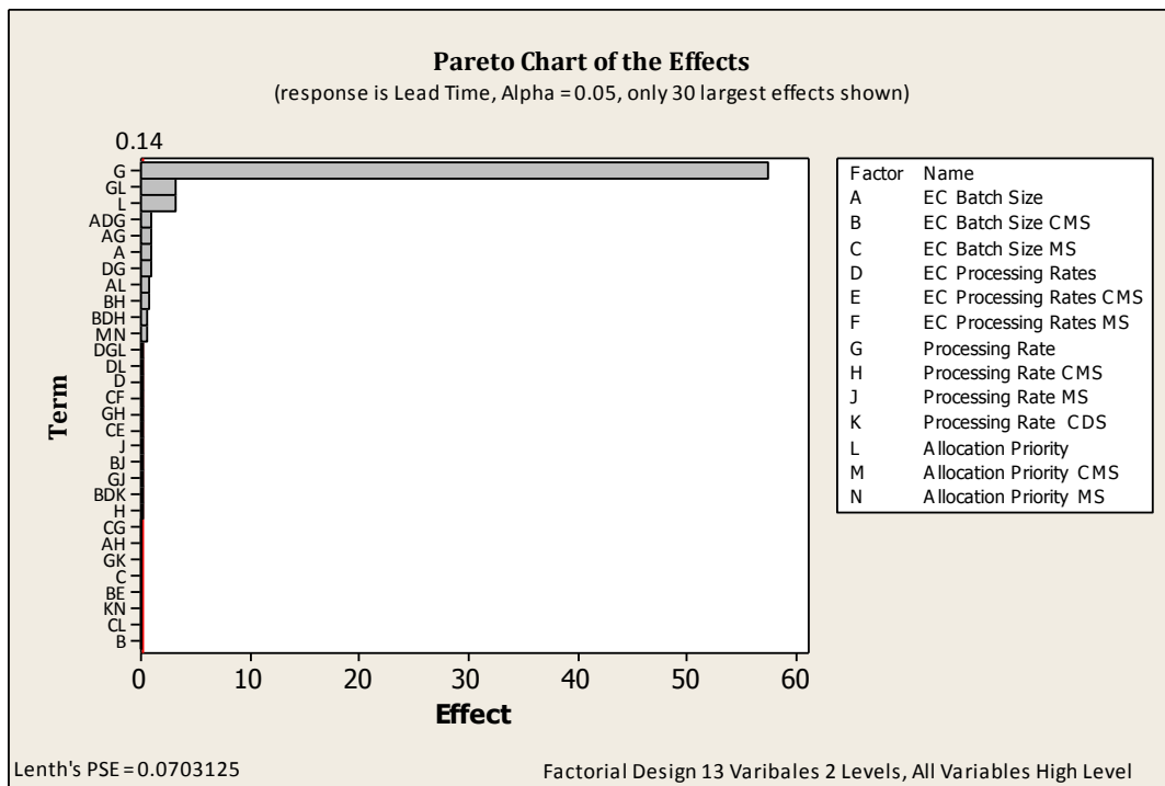
Figure 49: Pareto chart showing the effects of selected 13 factors on lead time with all variables at High state.
