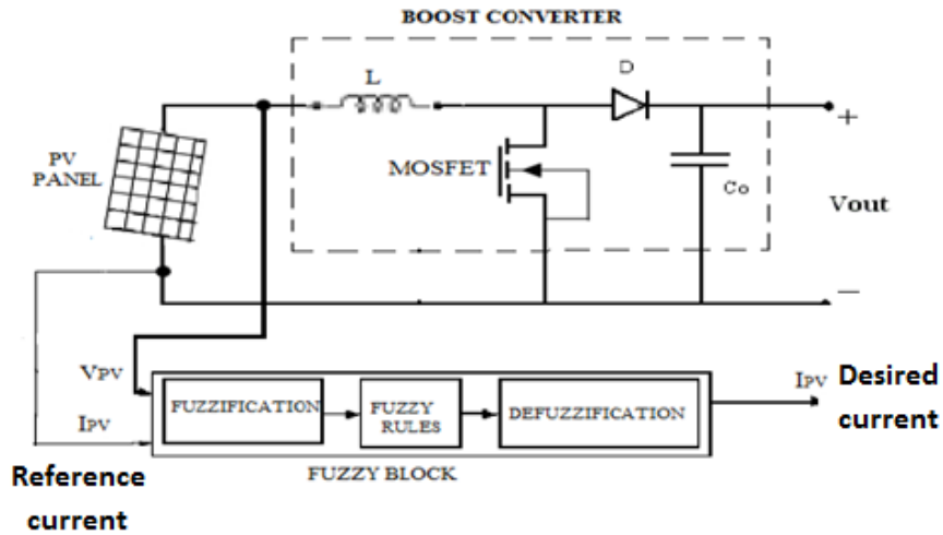
Figure 4.9: FLC controller
