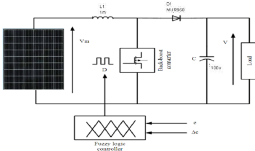
Figure 4.8: The block diagram of proposed PV control system
