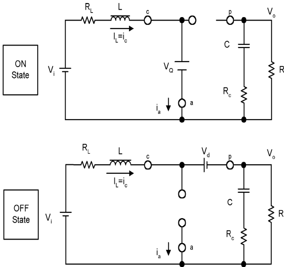
Figure 3.9: Boost Power Stage States
