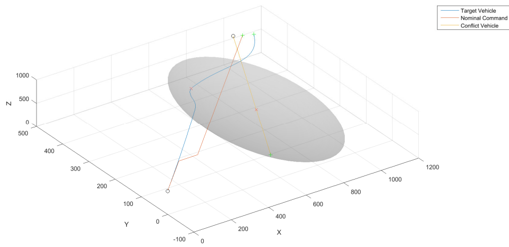
Figure 5.14 3D View; Instantaneous Jump in X
