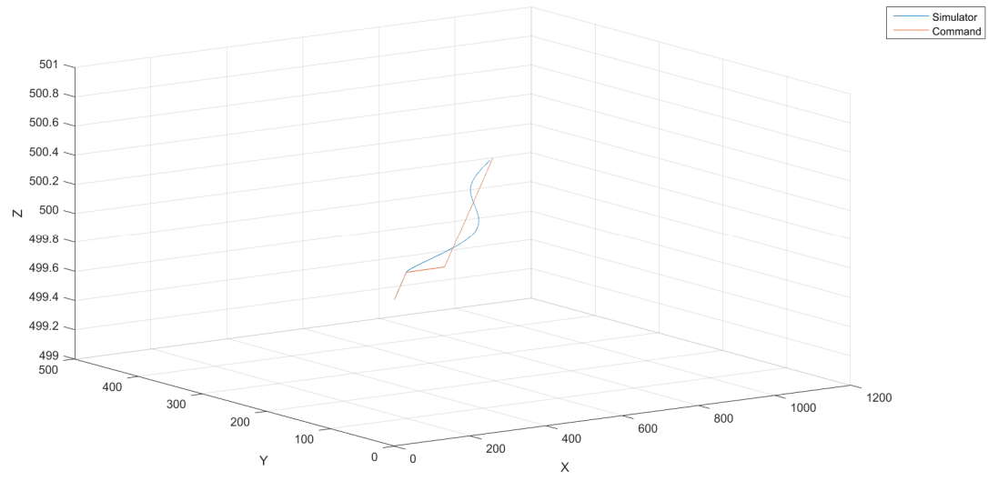
Figure 4.11 3D View of Trajectory with Instantaneous Jump in X
