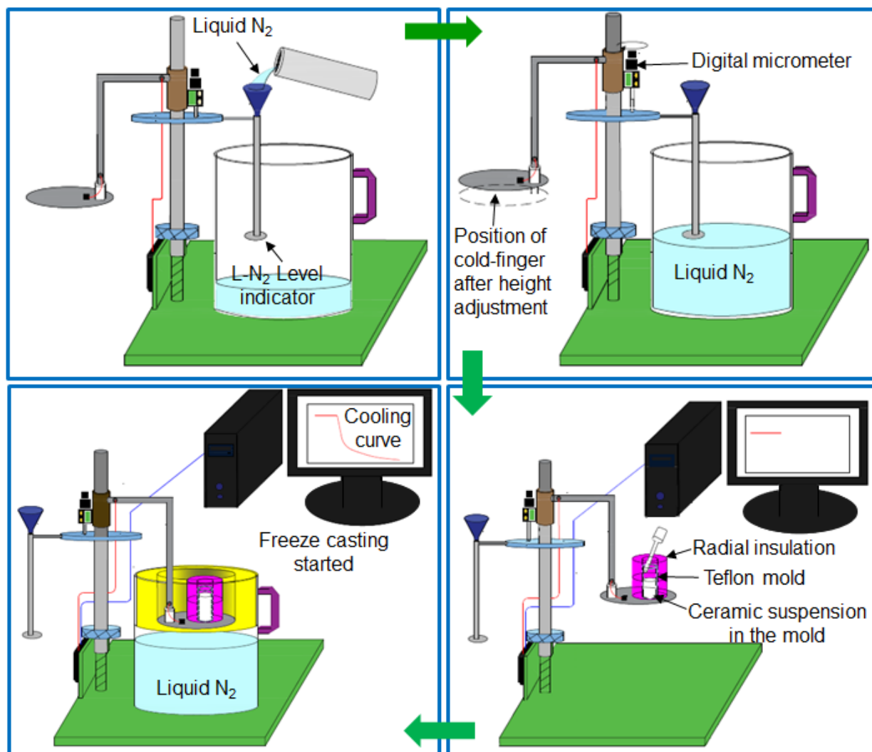
Figure 3.4: Schematic representation of the step-by-step operational procedure of the unidirectional freeze casting set up. (a) pouring of L- N_2 in to the Dewar, (b) adjustment of gap between L- N_2 and cold finger by digital micrometer, (c) transfer of ceramic slurry in to Teflon mold, (d) start of freeze casting experiment.
