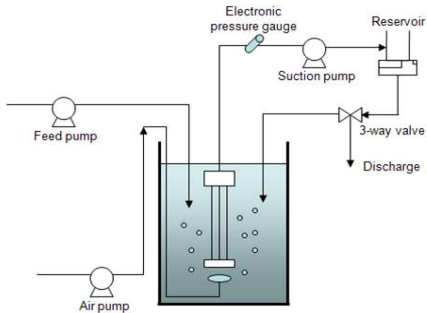
Figure 3.5 – Schematic of MBR
