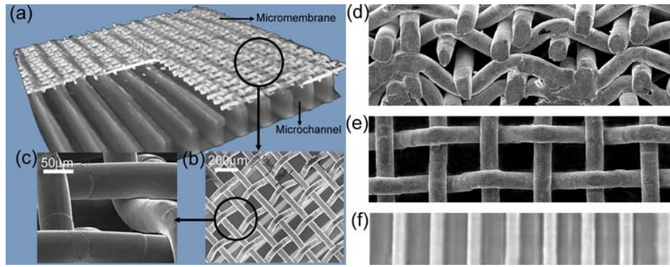
Figure 4.2 The micromembrane-enhanced evaporating surfaces developed in this study. (a) Three dimensional (3D) Micro-XCT image of the micromembrane-enhanced evaporating surface. (b) Top view of the micromembrane-enhanced evaporating surface. (c) Sharp corners formed by individual wires. (d) Sintered four-layer copper woven mesh laminates. (e) Single-layer mesh. (f) 3D Micro-XCT image of microchannels.
