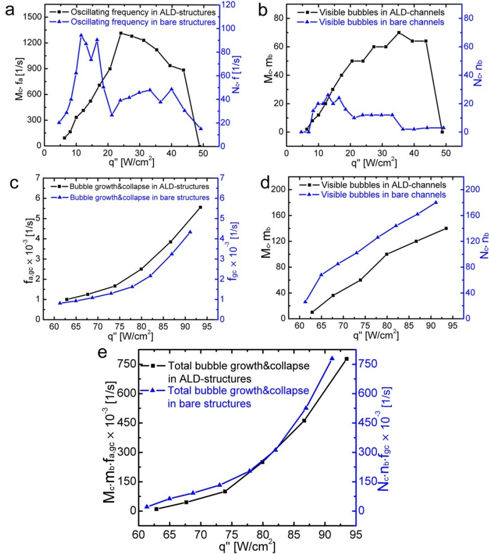
Figure 5.7 Comparisons of oscillating flows on the ALD SiO 2 coated and bare hybrid wicks (a) The total oscillating frequency, M_c \cdot f_a , on the ALD SiO 2 coated micromembrane-enhanced hybrid wicks; M_c is the number of active channels; and f_a is the frequency of fluid flow in a single active channel. N_c \cdot f is for the bare structure. (b) The total number of visible bubbles in active channels, M_c \cdot m_b . M_c is the number of
