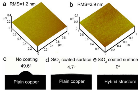
Figure 5.3 Characterization of the ALD SiO 2 coating. (a) 3-D AFM image of bare copper mesh. (b) 3-D AFM image of the conformal SiO 2 ALD coated copper mesh. (c) Contact angle on bare copper sheet. (d) Contact angle on ALD coated copper sheet. (e) Contact angle on ALD coated hybrid structure.
