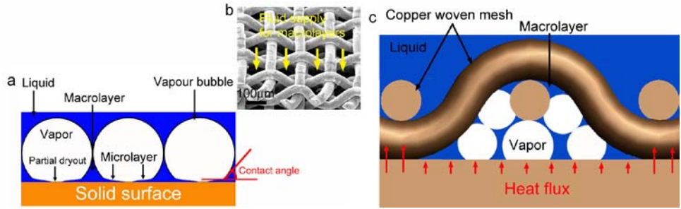
Figure 2.7 Heat transfer mechanisms. (a) Macrolayer & microlayer for nucleate boiling. (b) Fluid supply for the macrolayers in porous structures. (c) Macrolayer formation in two layer meshes.
