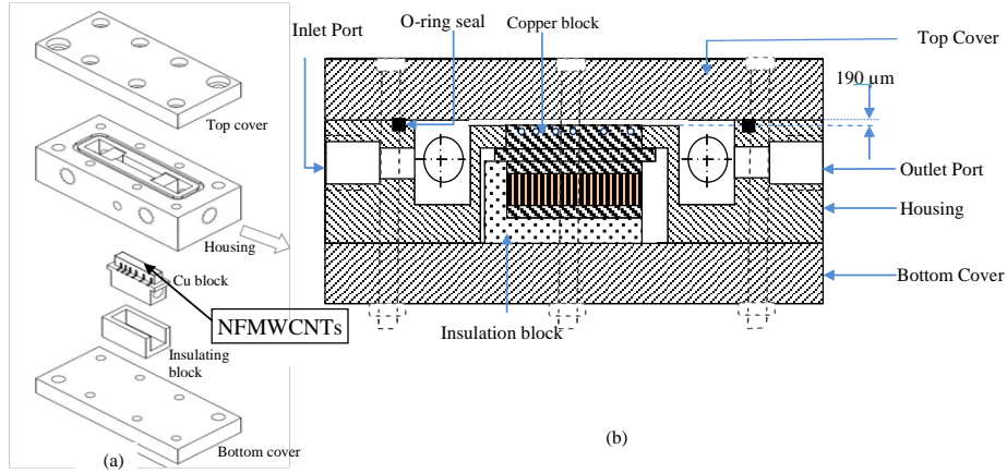
Figure A.7 (a) Test setup assembly. (b) Side view of the test sample and flow direction. pressure transducer (OMEGADYNE, INC. PX409, 0-15 PSI) was used to measure the pressure drop between the inlet and outlet plenums. The temperature and pressure signals were recorded by an Agilent 34972A data acquisition system.
