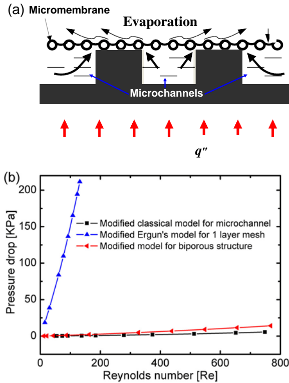
Figure 4.1 (a) Design of micromembrane-enhanced evaporating surfaces. (b) Comparisons of flow resistances between meshes, microchannels and the micromembrane-enhanced evaporating surfaces.
