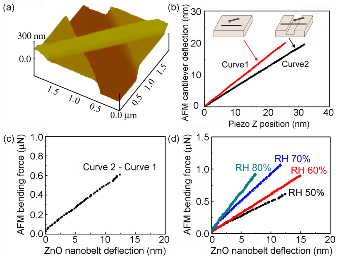
Figure 2.2 (a) The 3-D AFM image showing a ZnO nanobelt over the trench on the Si wafer. (b) Cantilever deflection as a baseline (curve 1) was obtained by performing three-point bending using an AFM tip directly. (c) Applied bending force as a function of net nanobelt deflection. (d) Applied bending force as a function of net nanobelt deflection under different relative humidity (RH) levels.
