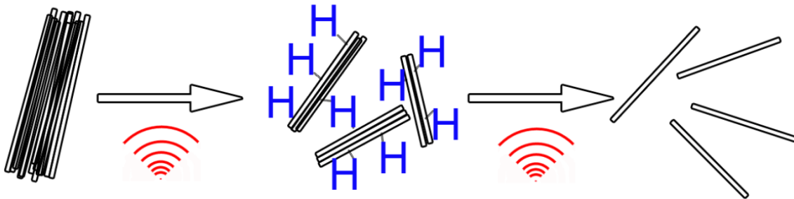
Figure 4.5 Schematic of MWCNT dispersion process with coupled HP and ultrasonication.
