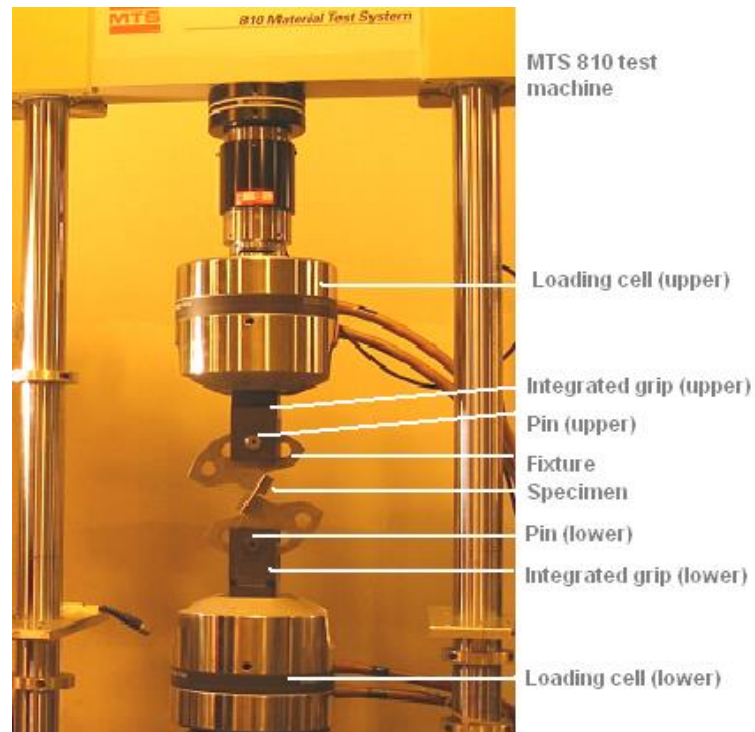
Fig. 2.5 The experimental system for the quasi-static, mixed-mode I/III tests.
