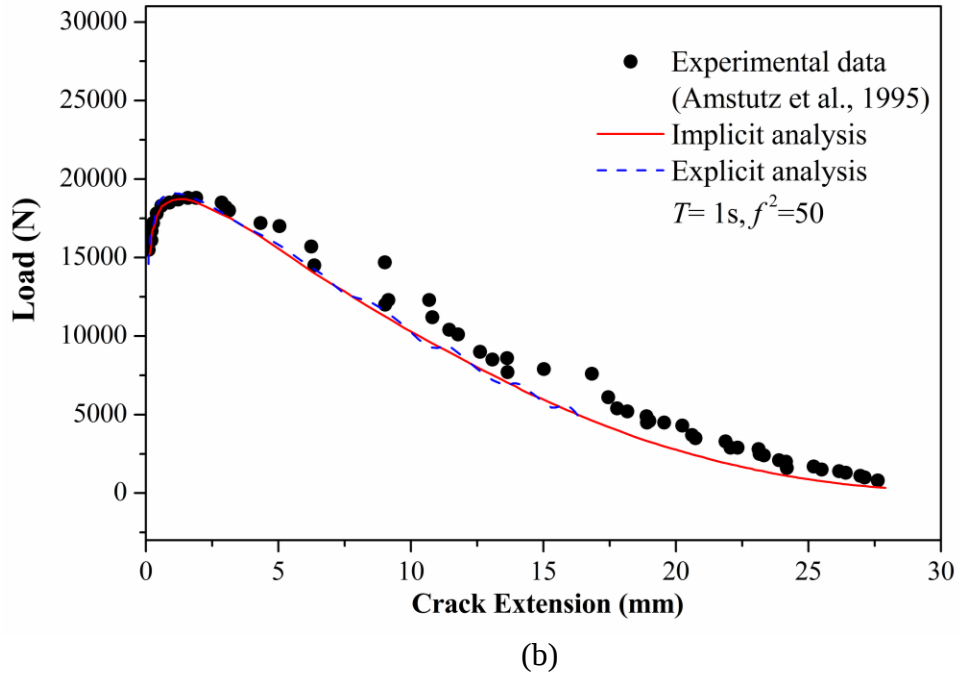
Fig. 4.7 (a) Convergence of the load-crack extension curve as the value of parameter f^2 decreases (with T=1\text{s} and \delta t = 4.0 \times 10^{-8}\text{s} ); (b) Comparison of converged predictions of the load-crack extension curve using the explicit procedure (with T=1\text{s} , \delta t = 4.0 \times 10^{-8}\text{s} and f^2=50 ) and the implicit procedure with experimental measurements (Amstutz et al., 1995).
