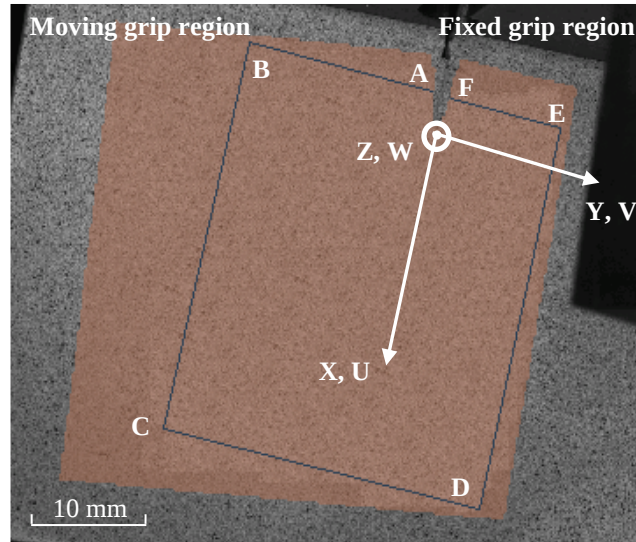
Fig.7.1 A surface image of an un-deformed mixed-mode I/III 6061-T6 aluminum alloy specimen loaded at 60°, showing a sub-region, the coordinate system with origin at the pre-crack tip, and lines for data comparison.
