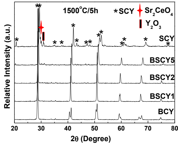
Figure 3.2 XRD patterns of Ba 1-x Sr x Ce 0.8 Y 0.2 O 3-δ (BSCY, x=0, 0.1, 0.2, 0.5 and 1, denoted as BCY, BSCY1, BSCY2, BSCY5 and SCY, respectively) sintered at 1500°C for 5h in air.
