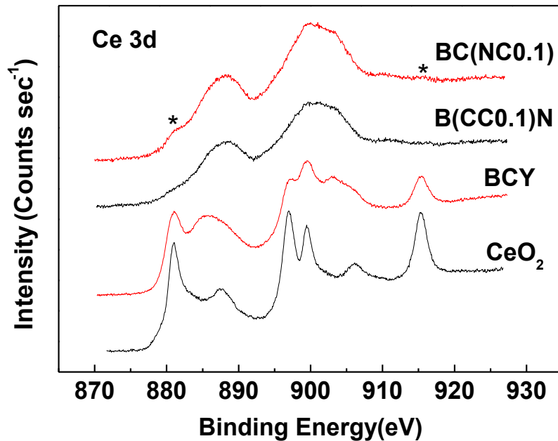
Figure 3.18 XPS spectra of Ce 3d for samples BC(NC0.1), B(CC0.1)N, BaCe 0.85 Y 0.15 O 3- \delta (BCY) and CeO 2 collected at room temperature.
