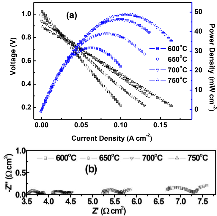
Figure 5.8 (a) Cell voltage and power density as a function of current density for Ni-BCN18|BCN18|BCFN single cell fabricated by conventional sintering method at 1400°C for 5h, and (b) impedance spectra of the single cell under open-circuit conditions.
