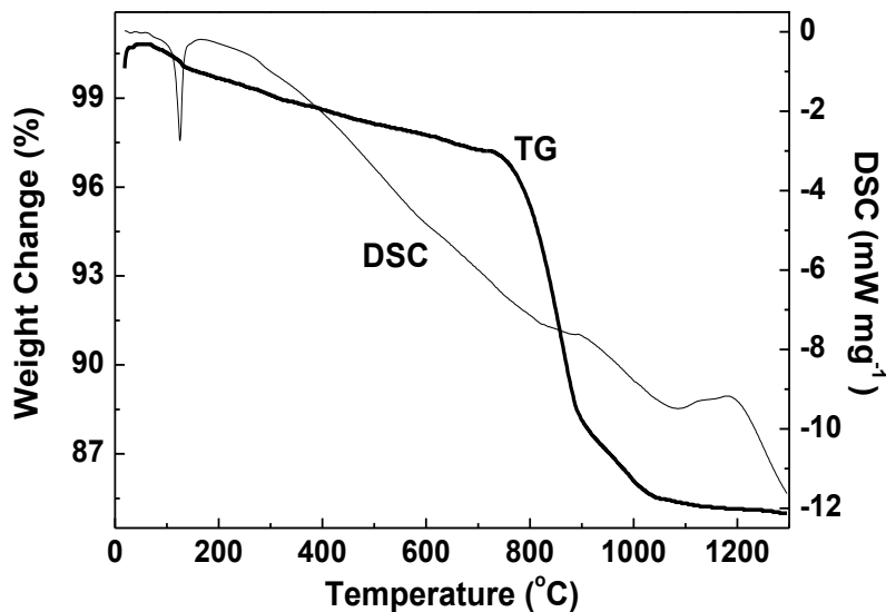
Figure 3.6 TG-DSC curves of the BZCYYb powder preheated at 600°C for 4 h.
