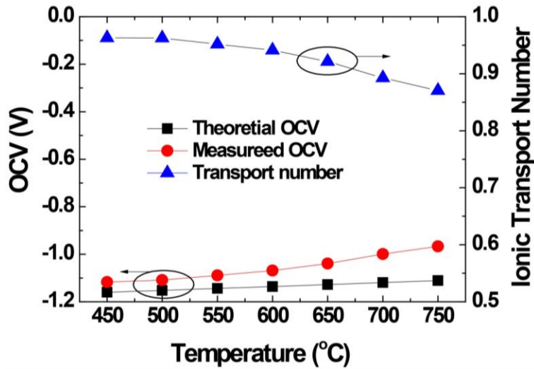
Figure 4.17 Theoretical and measured OCV values for BCNY0.3 with 3vol%H 2 O-H 2 /Pt | BCNY0.3 | Pt/Air and ionic transport number.
