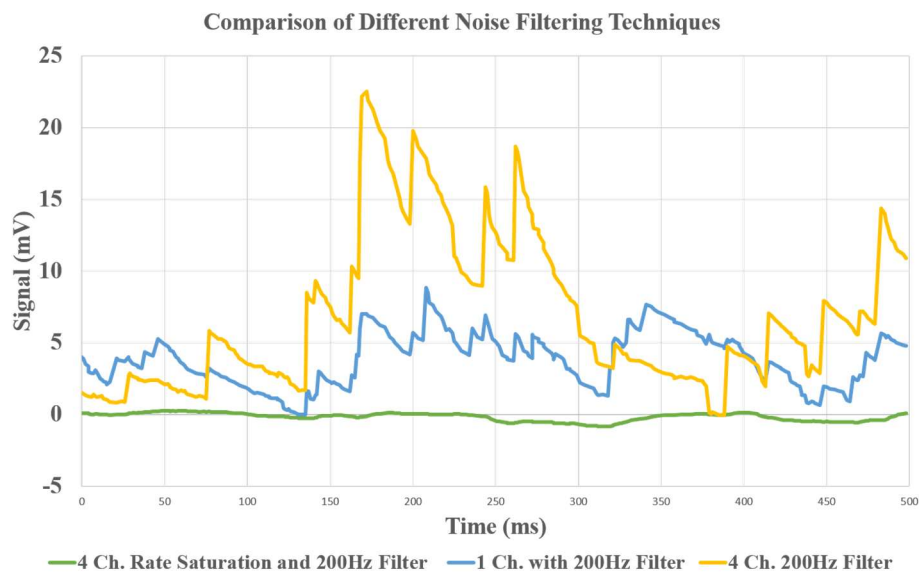
Figure 23: Noise in Load Cell Signal Filtered Using Different Methods
