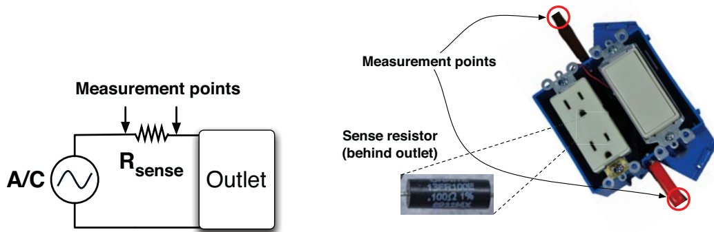
(a) A circuit diagram of our measurement technique. The difference in voltage on either side of the resistor ( R_{sense} ) is proportional to the power consumed by the AC device at left. The same measurement technique applies to DC circuits.
