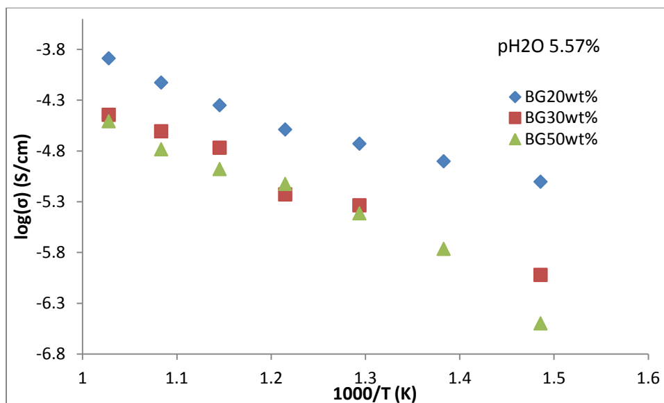
Figure 2.20 Arrhenius plot of ionic conductivity for BG 20wt%, 30wt%, and 50wt% under 5.57% pH 2 O.
