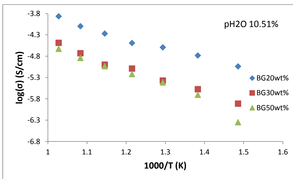
Figure 2.21 Arrhenius plot of ionic conductivity for BG 20wt%, 30wt%, and 50wt% under 10.51% pH 2 O.
