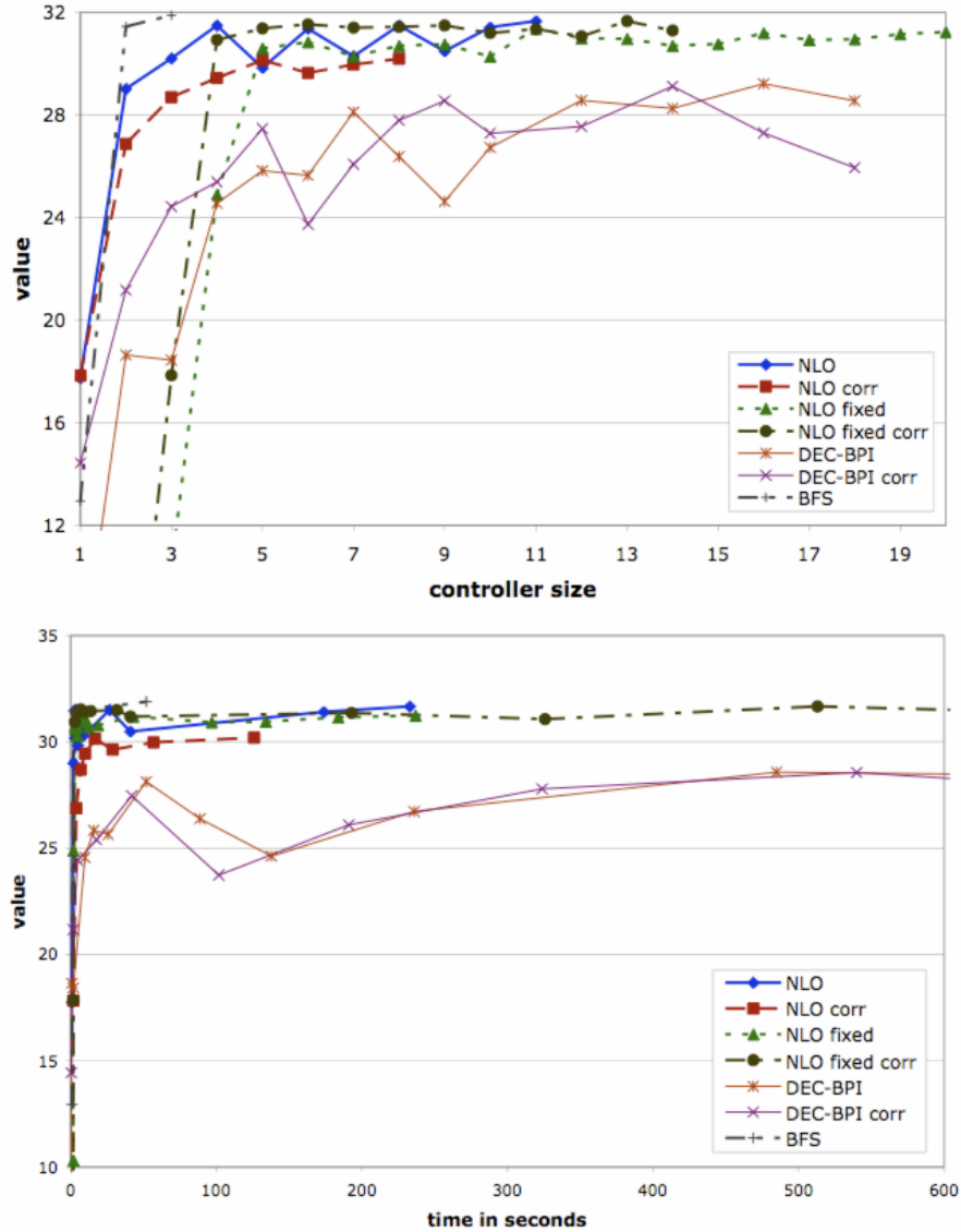
Figure 5.2. Recycling robots values for various controller sizes (top) and running times (bottom) using NLP methods and DEC-BPI with and without a 2 node correlation device and BFS
