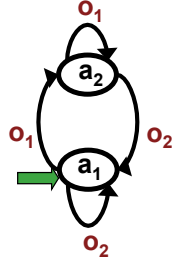
Moore Machine
