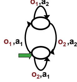
Mealy Machine
