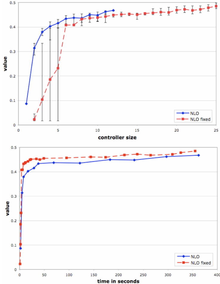
Figure 5.1. Hallway problem values for various controllers sizes (top) and running times (bottom) using the NLP formulation with and without fixed actions at each node. Bars are used in the left figure to represent the minimum and maximum values for each size.
