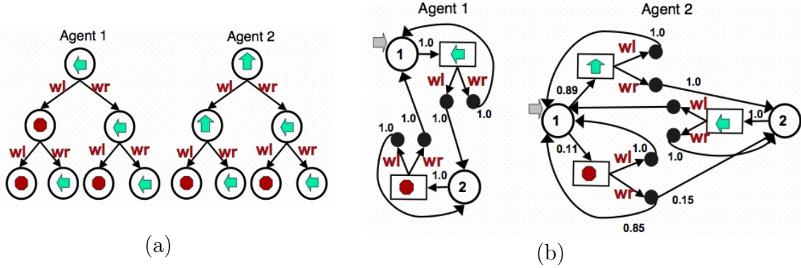
Figure 3.1. A set of horizon three policy trees (a) and two node stochastic controllers (b) for a two agent DEC-POMDP.
