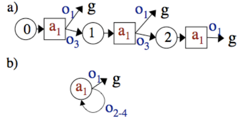
Figure 8.1. An example of a controller generated from a set of trajectories. The trajectories all begin at an initial state and end when a goal condition has been satisfied. The initial controller is then created from these trajectories and redundant nodes are combined to produce the reduced controller. This controller is then optimized by evaluating it in conjunction with the controllers of the other agents and optimizing the action choices and transition choices as shown in a) and b) respectively.
