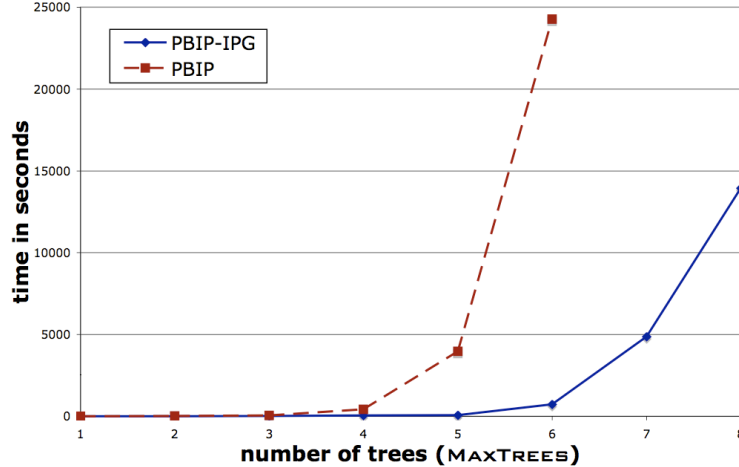
Figure 7.2. Running times for different values of MAXTREES on the Box Pushing problem with horizon 10.
