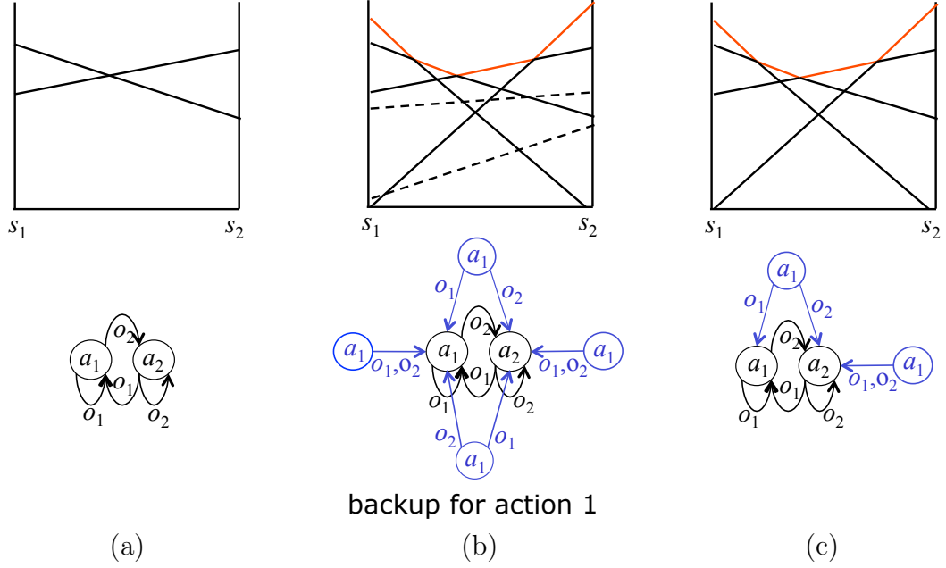
Figure 2.4. Controllers and value vectors in policy iteration: the previous step controller (a), the backed up controller (for action 1 only) (b), and after pruning (c).
