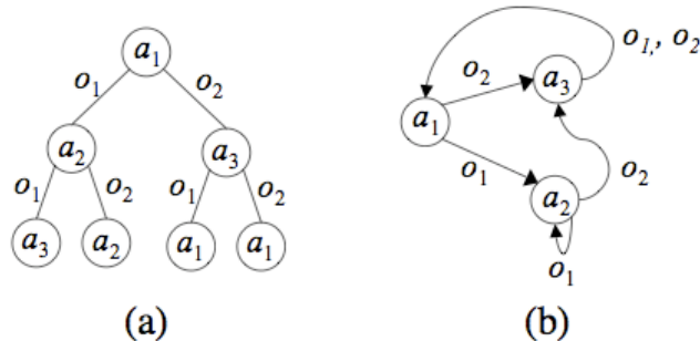
Figure 2.1. Examples of POMDP policies represented as (a) a policy tree and (b) a deterministic finite-state controller.
