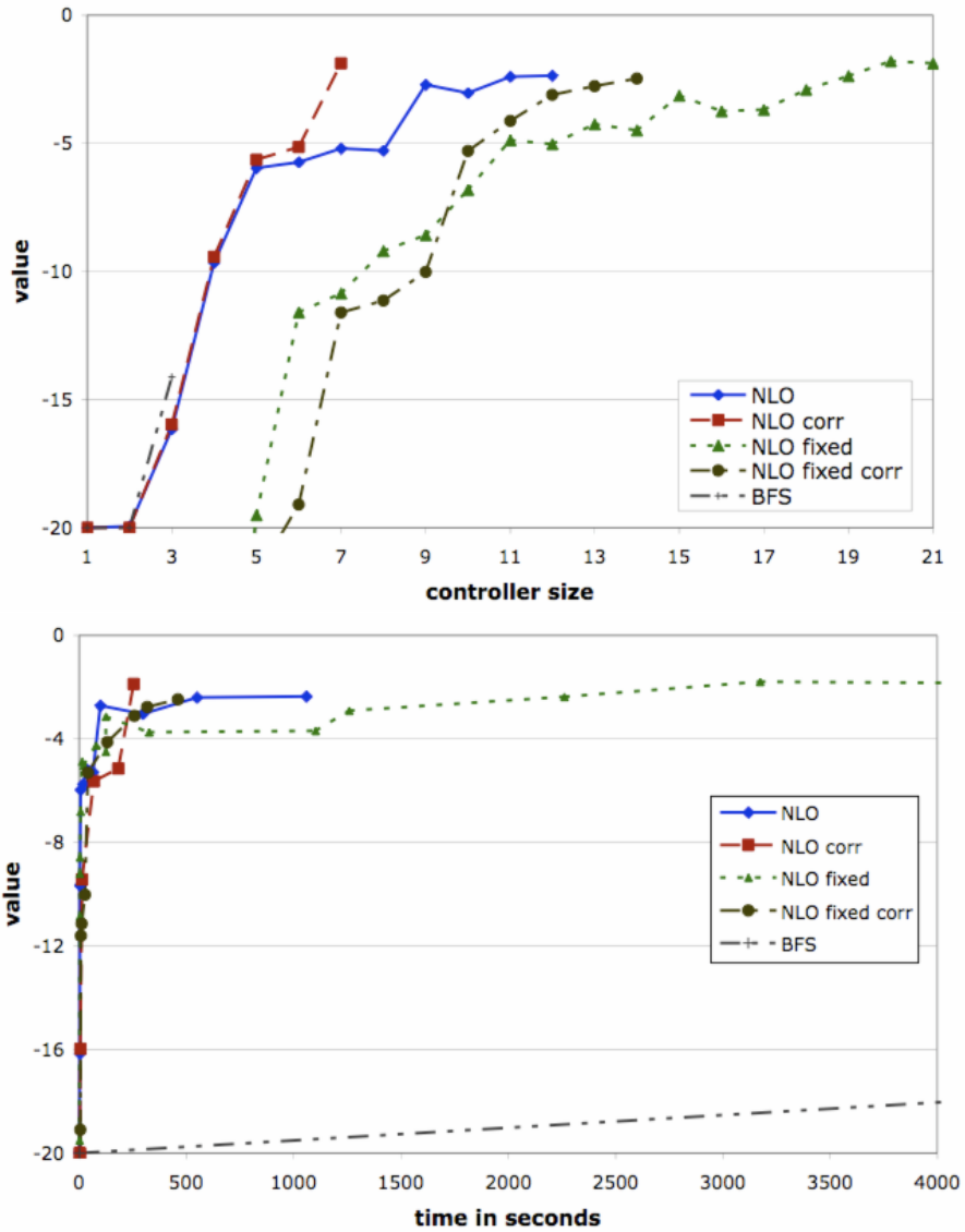
Figure 5.3. Multiagent tiger problem values for various controller sizes (top) and running times (bottom) using NLP methods with and without a 2 node correlation device and BFS
