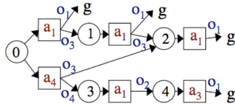
Figure 8.1. An example of a controller generated from a set of trajectories. The trajectories all begin at an initial state and end when a goal condition has been satisfied. The initial controller is then created from these trajectories and redundant nodes are combined to produce the reduced controller. This controller is then optimized by evaluating it in conjunction with the controllers of the other agents and optimizing the action choices and transition choices as shown in a) and b) respectively.
