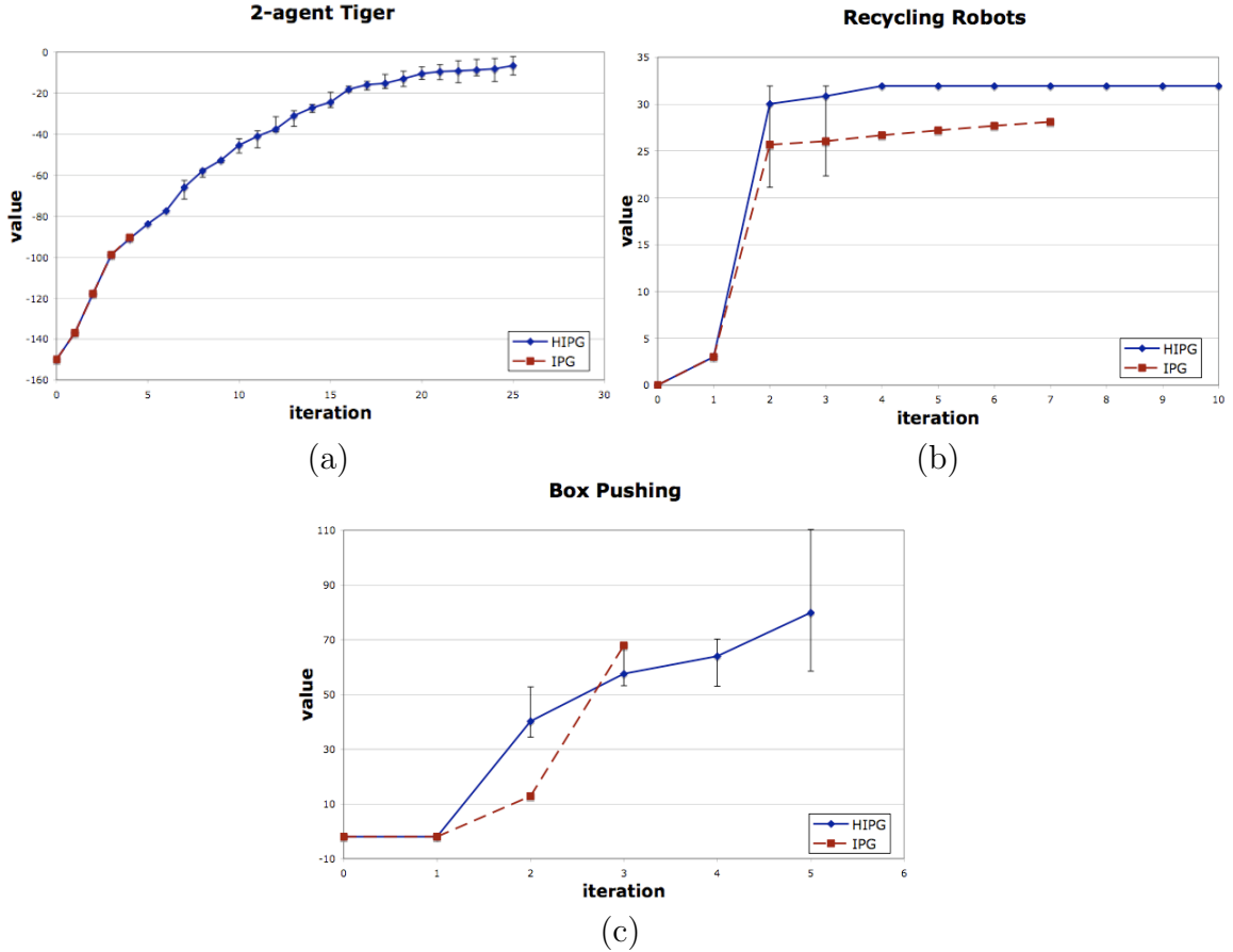
Figure 7.3. Comparison of the heuristic and optimal incremental policy generation algorithms on (a) the two agent tiger, (b) recycling robot and (c) the box pushing problems.
