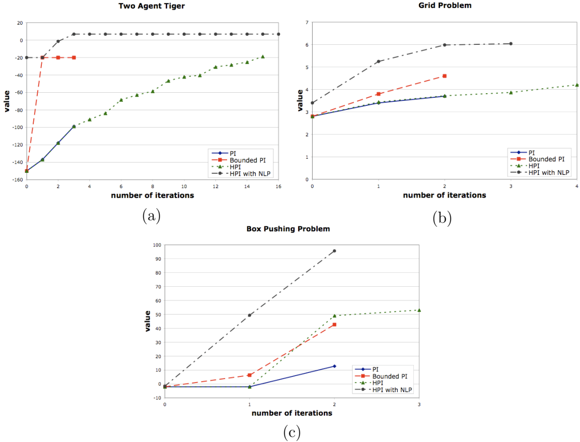
Figure 7.1. Comparison of the dynamic programming algorithms on (a) the two agent tiger problem, (b) the meeting in a grid problem and (c) the box pushing problem. The value produced by policy iteration with and without bounded backups as well as our heuristic policy iteration with and without optimizing the NLP were compared on each iteration until the time or memory limit was reached.
