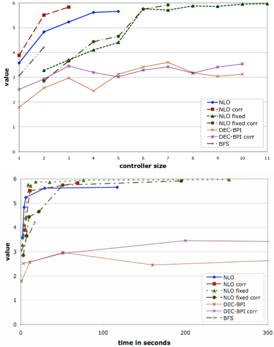
Figure 5.4. Meeting in a grid problem values for various controller sizes (top) and running times (bottom) using NLP methods and DEC-BPI with and without a 2 node correlation device and BFS
