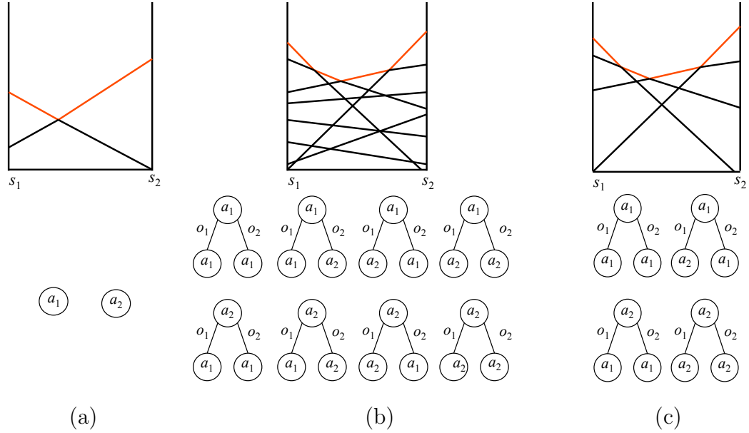
Figure 2.3. Policy trees and value vectors in value iteration: the first step (a), the second step, an exhaustive backup (b), and after pruning (c).
