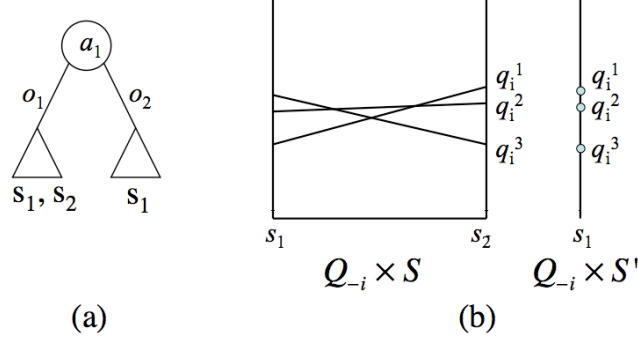
Figure 4.1. Example of (a) limiting states after actions are chosen and observations seen and (b) pruning with a reduced state set, S' .
