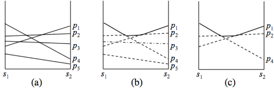
Figure 2.2. Value vector illustrations for a problem with 2 states. In (a) the values for policies p_1 - p_5 is presented. In (b), the maximum value for all belief states is highlighted. In (c) only policies that contribute to this maximum value are retained and the remaining policies are pruned.
