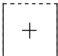
State 8 – [0111]
