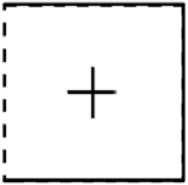
State 15 – [1110]
