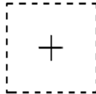
State 1 – [0000]
