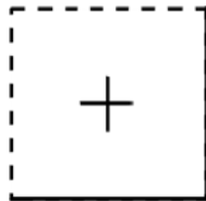
State 7 – [0110]
