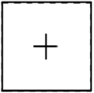
State 16 – [1111]
