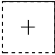
State 13 – [1100]
