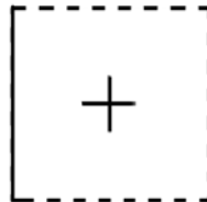
State 2 – [0001]
