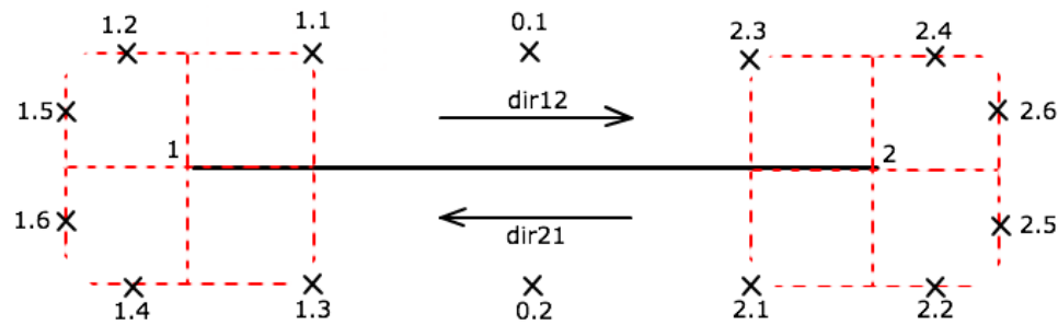
Figure 4.6: Reference Points to Relevant Building Structure
