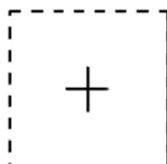
State 5 – [0100]
