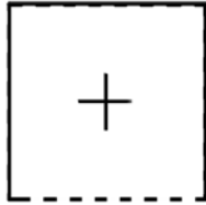
State 14 – [1101]
