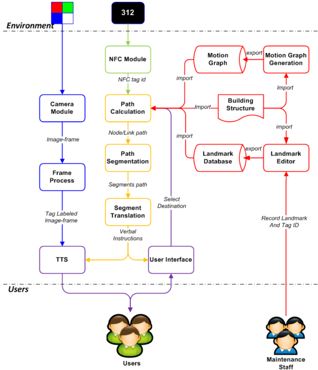
Figure 1.3: System Architecture
