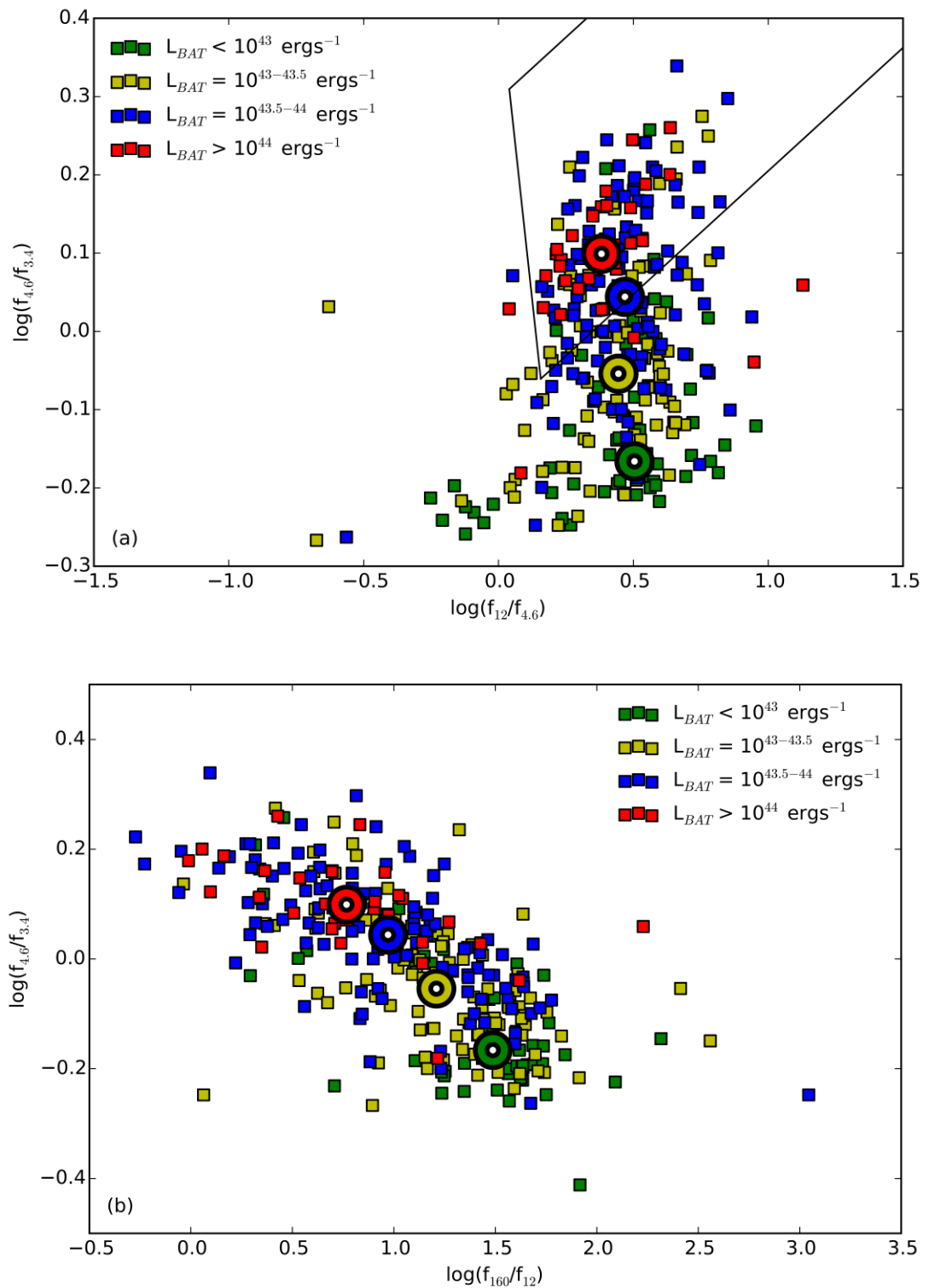
Figure 2.10: Colour-colour plots for Swift -BAT AGN sample with AGN selection based on the Swift -BAT X-ray luminosity, L_{BAT} . Top: Mid-infrared colour selection with an AGN wedge as defined from Mateos et al. (2012) for luminous X-ray detected AGN using WISE wavebands. Bottom: Mid-to-far-infrared colour selection that demonstrates the use of both WISE and Herschel waveband photometry. The larger filled circles with white dots are averages for each bin of BAT luminosity.
