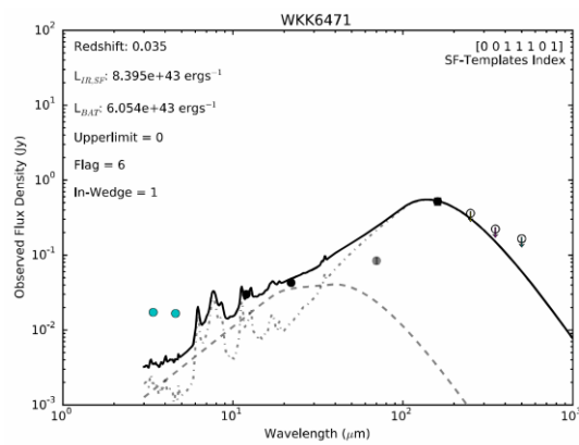
Figure A.41: Continued from Figure A.2, Best-fitted SED solution for one of the Swift -BAT sources (listed alphabetically).
