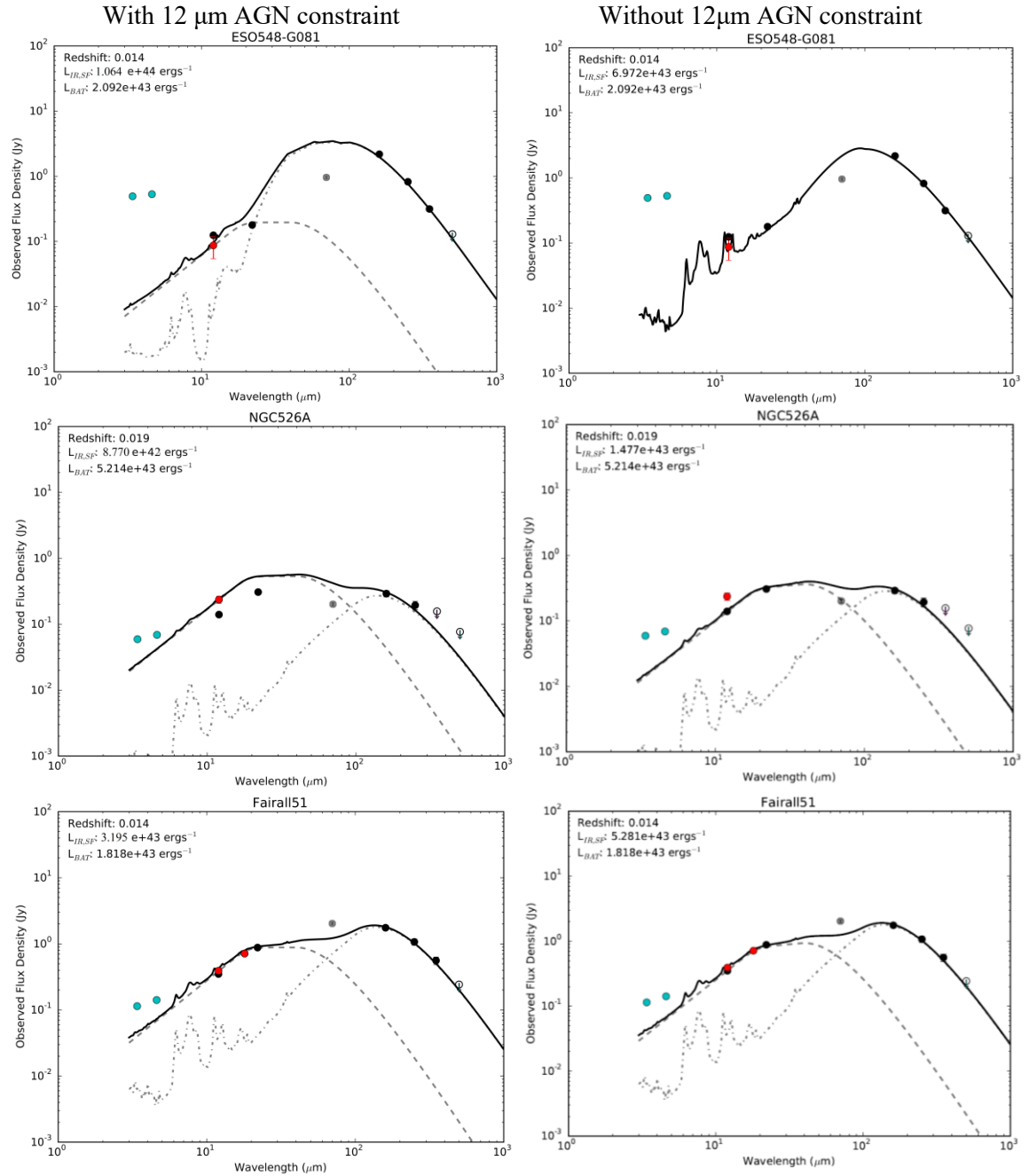
Figure 2.7: Best-fitting SED solutions for ESO548-G081, NGC 526A and Fairall 51, the three largest outliers from Figure 2.6. Left: The AGN template is fixed to the subarcsecond resolution 12 \mu\text{m} photometry (Asmus et al. 2014). Right: The AGN template is left as a free parameter in the SED fitting procedure. In all six cases the black filled data points are measured flux densities from Herschel (160 – 500 \mu\text{m} ) and WISE (12 and 22 \mu\text{m} ) observations, the cyan filled data points are measured flux densities from WISE (3.4 and 4.6 \mu\text{m} ) observations, the red data points are measured subarcsecond-resolution mid-infrared (12 and 18 \mu\text{m} wherever possible) photometry from Asmus et al. (2014), the grey data points are flux densities from Herschel at 70 \mu\text{m} and are not used in the fitting procedure (see Section 4.2), while the empty circles with a downward arrow are flux density upper limits.
