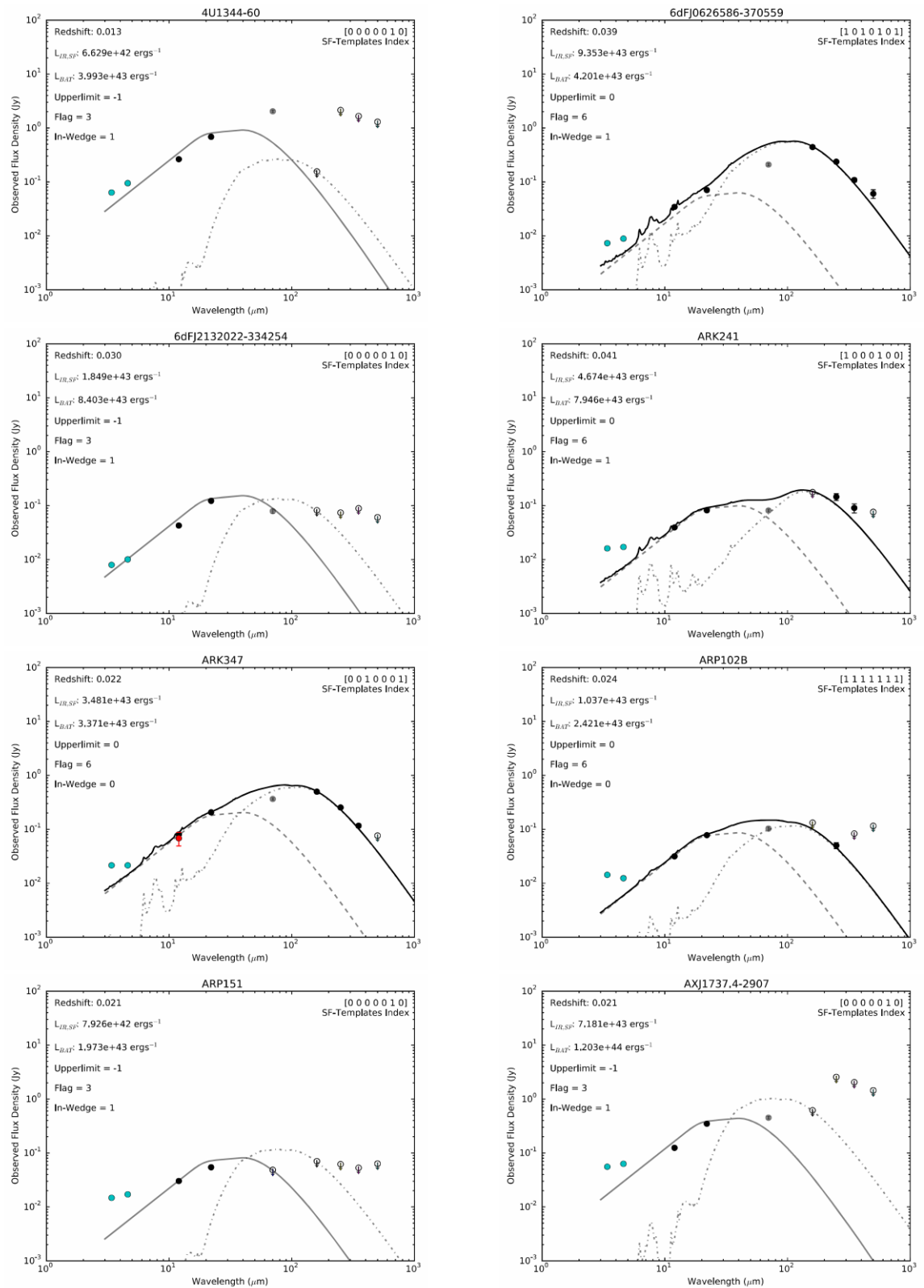
Figure A.9: Continued from Figure A.2, Best-fitted SED solutions for eight Swift -BAT sources (listed alphabetically).
