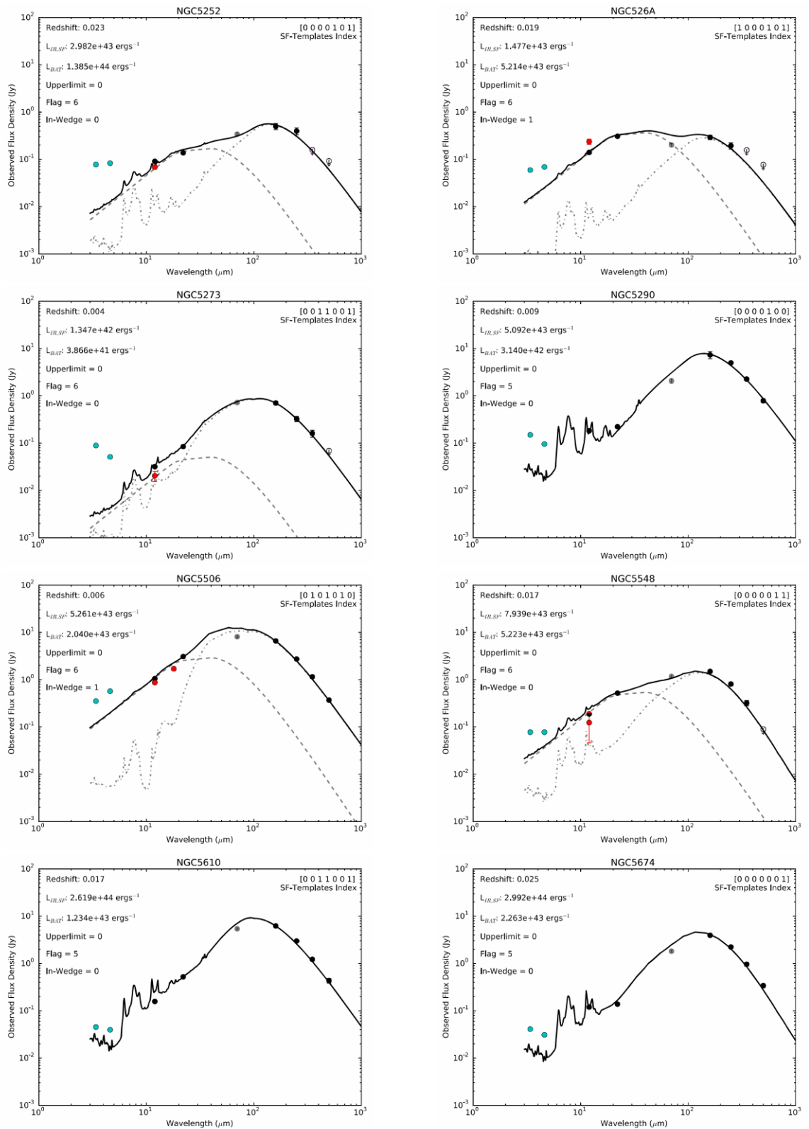
Figure A.34: Continued from Figure A.2, Best-fitted SED solutions for eight Swift -BAT sources (listed alphabetically).
