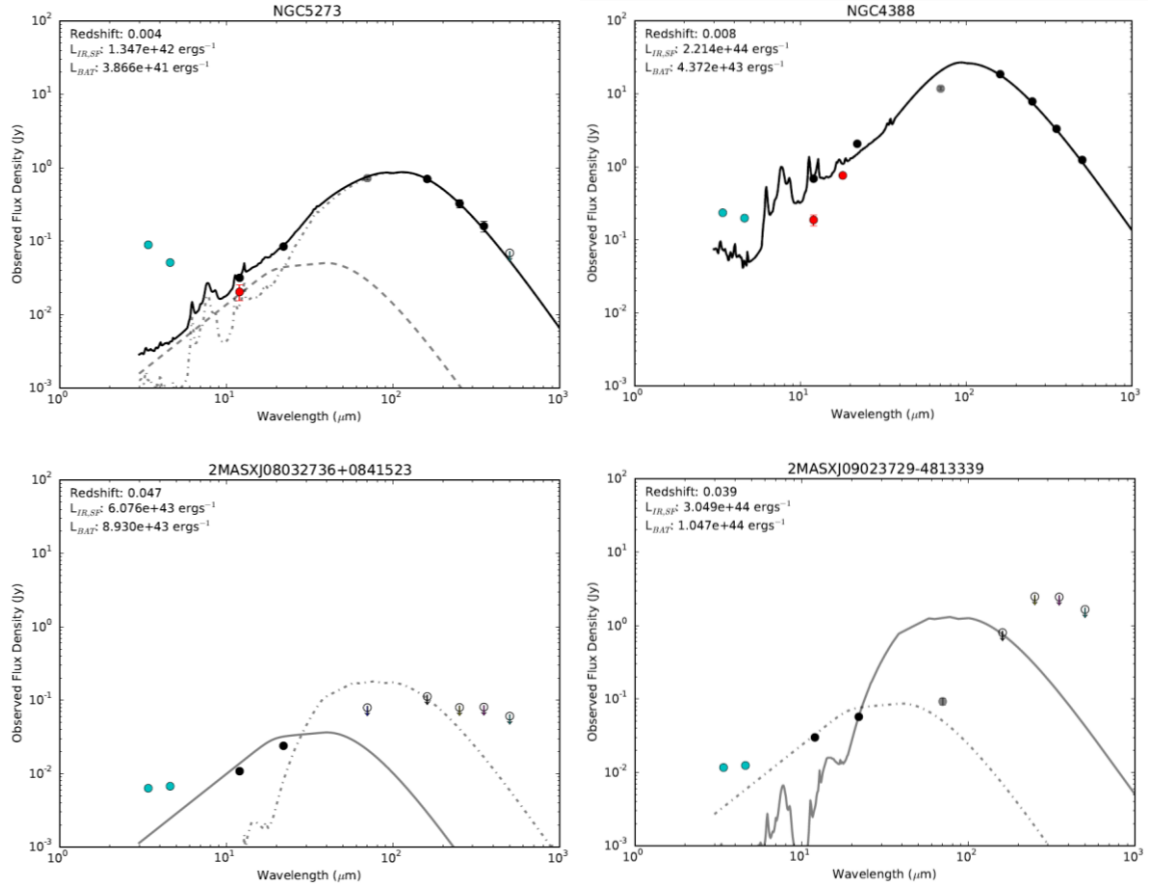
Figure 2.3: Four examples of our SED fits. In all four cases the black filled data points are measured flux densities from Herschel (160 – 500 \mu\text{m} ) and WISE (12 and 22 \mu\text{m} ) observations, the cyan filled data points are measured flux densities from WISE (3.4 and 4.6 \mu\text{m} ) observations, the red data points are measured subarcsecond-resolution mid-infrared (12 and 18 \mu\text{m} wherever possible) photometry from Asmus et al. (2014), the grey data points are flux densities from Herschel at 70 \mu\text{m} and are not used in the fitting procedure (see Section 4.2), while the empty circles with a downward arrow are flux density upper limits. Additionally, we provide the infrared luminosity due to star formation ( L_{\text{IR,SF}} ), the BAT (14-195 keV) X-ray luminosity ( L_{\text{BAT}} ), the redshift and the name of each source. Errors for the measure flux densities are provided but may be small. (a) The best fitting (black solid) SED solution is a combination of AGN (grey dashed) and star forming (grey dot-dashed) galaxy templates. (b) The best fitting (black solid) SED solution is that of a star-forming galaxy template with no AGN contribution. (c) The best fitting SED solution is an AGN (grey solid) that has no star formation due to limited photometric detections, so in this case we provide an upper limit (grey dot-dashed) with the star forming galaxy template that does not exceed the 160 \mu\text{m} data point. (d) The best fitting SED solution is a star forming (grey solid) galaxy template with no AGN contribution due to limiting photometric detections, therefore we provide an upper limit to the AGN (grey dot-dashed) contribution that does not exceed the 160 \mu\text{m} data point.
