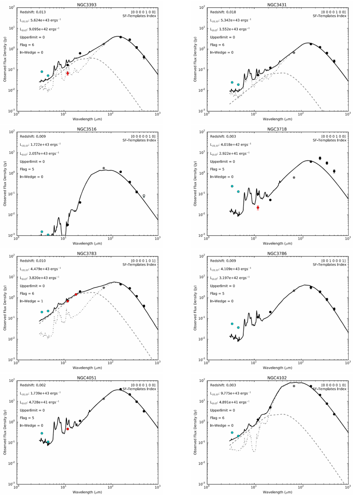
Figure A.31: Continued from Figure A.2, Best-fitted SED solutions for eight Swift-BAT sources (listed alphabetically).
