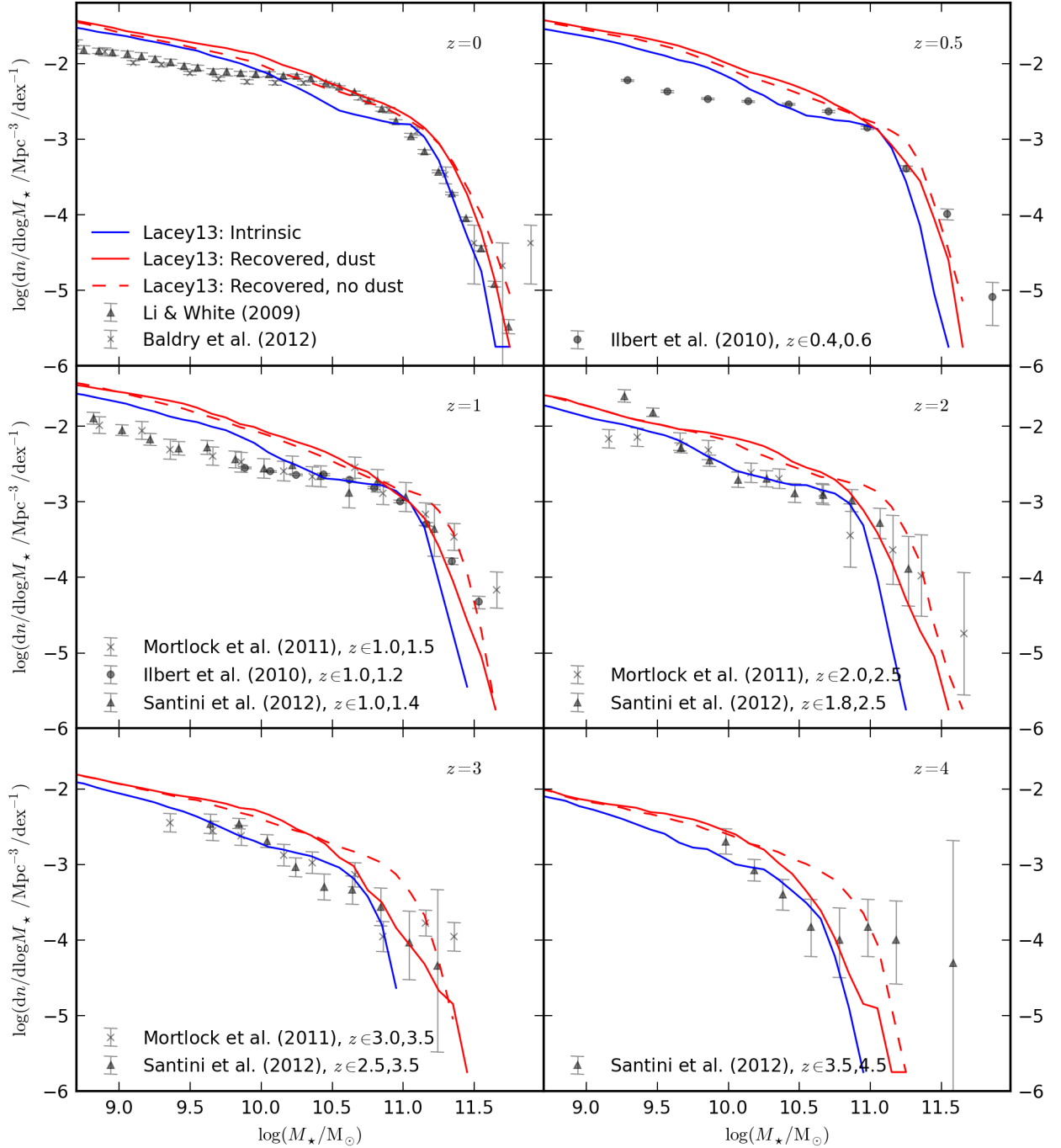
Figure 3.13: Stellar mass functions predicted by the Lacey13 model for a selection of redshifts, as labelled in each panel. The definition and formatting of the lines and points is the same as in Fig. 3.12.
