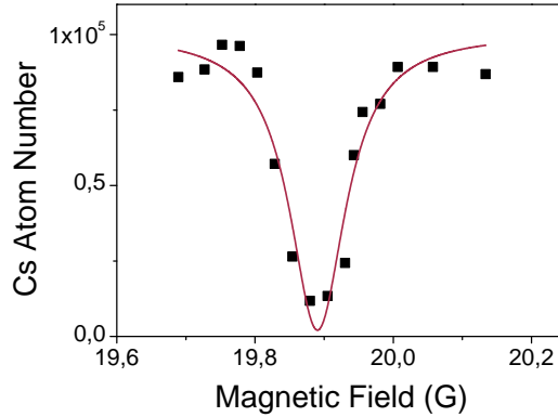
Figure 7.2: Cs Feshbach resonance at 19.89(2) G which is used to associate Cs 2 molecules. The position and width of 0.10(2) G are determined by a Lorentzian fit to the loss feature.
