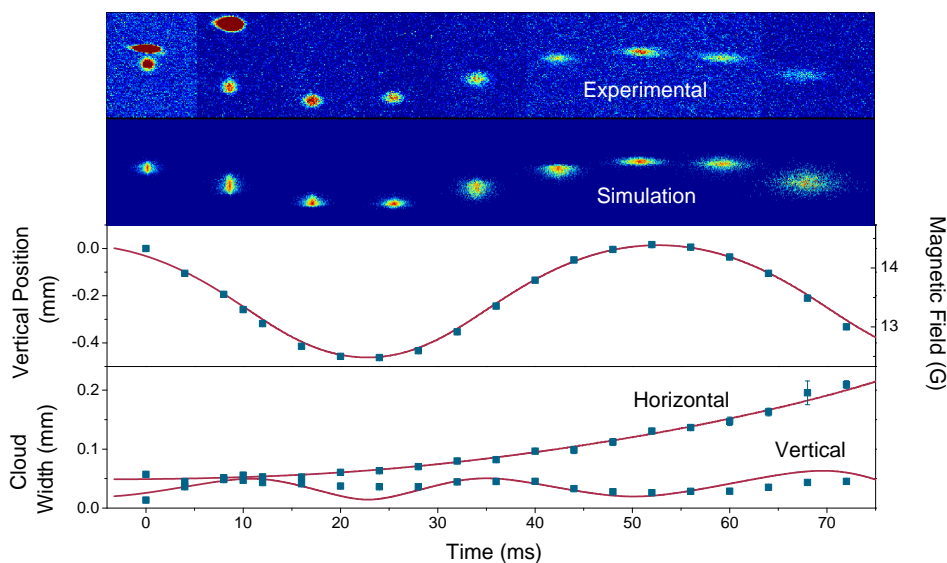
Figure 7.8: Position and shape of the molecular cloud versus time. The motion of the molecules is simulated in a quadrupole field with a magnetic field gradient of 40 G/cm and the potential presented in figure 7.7. In the top panel, absorption images and results of the simulation are presented. In the two panels below, the experimental data and results of the simulation of the cloud position and widths in the horizontal and vertical direction are shown.
