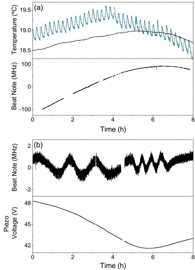
Figure 4.10: Drift of the home-built cavity over 8 hours. (a) Top panel: Room temperature (blue) and the temperature inside the vacuum chamber (black). The fast temperature change from the air-conditioning is filtered out and the maximum temperature is not as high inside the chamber. Bottom panel: Beat note between a laser locked to an atomic transition and one locked to a cavity mode. The laser locked to the cavity drifts \sim 400 MHz/K. (b) Top panel: Same beat note as in the graph above, but now the cavity length is stabilised by locking a cavity resonance to a Cs transition. The amplitude decreased to \sim 3 MHz. Bottom panel: Piezo voltage to keep the resonator length stable whilst the cavity is locked.
