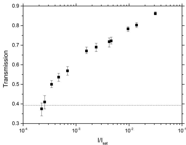
Figure 3.9: Transmission of the K D2 line measured at zero detuning as a function of I/I_{\text{sat}} for a 1 cm long K+Cs mixed species cell. The dashed line indicates the predicted transmission in the weak-probe regime, determined from measurements at the lowest probe intensities.
