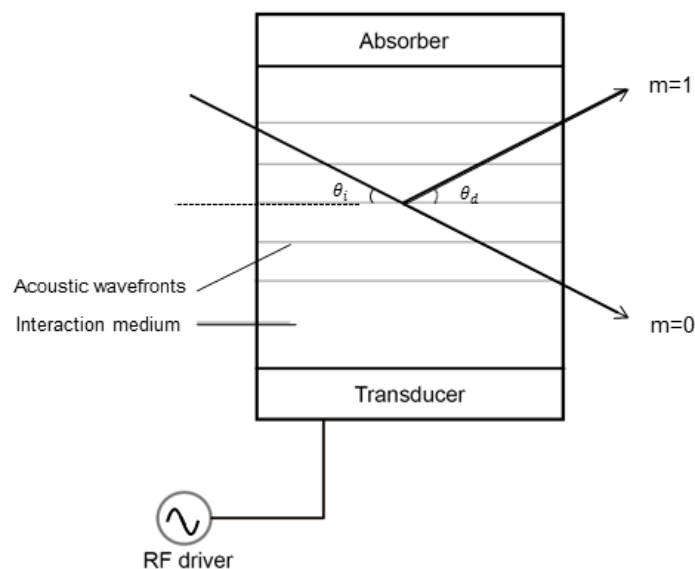
Figure 5.1: Schematic of an acousto-optic modulator. The signal from an RF driver is converted into acoustic waves which is passed into the interaction medium. The acoustic wavefronts act as gratings from which the incident laser beam with an angle \theta_i is deflected into the 1 st ( m=1 ) order with an angle \theta_d from the normal. m=0 corresponds to the undeflected light.
