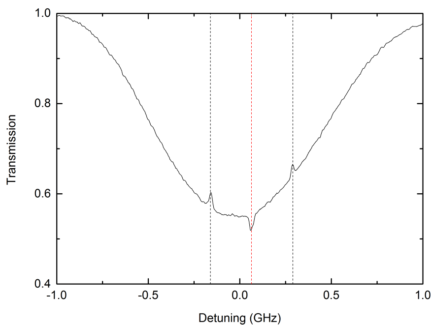
Figure 3.13: Transmission plotted against linear detuning of a pure, 10 cm potassium cell used as a reference for getting the ECDL on the K D2 transition. The approximate temperature of the cell as measured with a thermocouple is 35^{\circ}\text{C} . The black dashed lines indicate the F = 1 and F = 2 hyperfine splitting and the red dashed line shows the crossover dip occurring halfway between the F = 1 and F = 2 levels.
