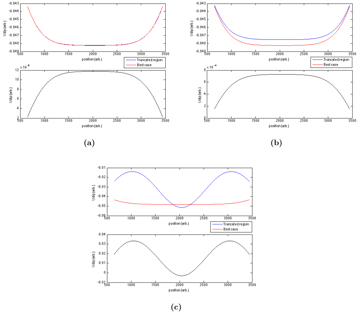
Figure 6.7: The top subplot of (a)-(c) show the trapping potential of the truncated region (blue) and the best case potential having 1001 Gaussians (red). The bottom subplot show the residuals for each corresponding to labels (A)-(C) in Fig. 6.5. The s/w_0 value of (a)-(c) are 9.77 \times 10^{-4} (2049 Gaussians), 59.00 \times 10^{-4} (65 Gaussians), 107.00 \times 10^{-4} (3 Gaussians), respectively. The RMS values over the truncated region for (a)-(c) are 0.02%, 1.31%, and 47.55%, respectively.
