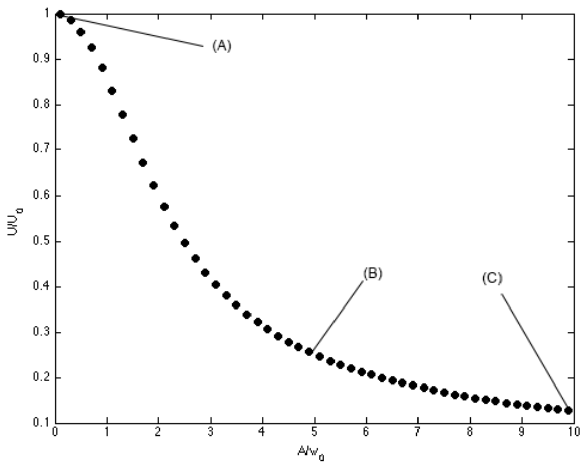
Figure 7.2: U/U_0 vs. A/w_0 where A is the dither range, w_0 is the beam waist, U is the minimum trap depth of the dithered trapping potential and U_0 is the minimum trap depth of the undithered potential. (A)-(C) correspond to an A/w_0 value of 0.1, 4.9, and 9.9, respectively. Note: labels (A)-(C) correspond to potentials (A)-(C) in Fig. 7.1.
