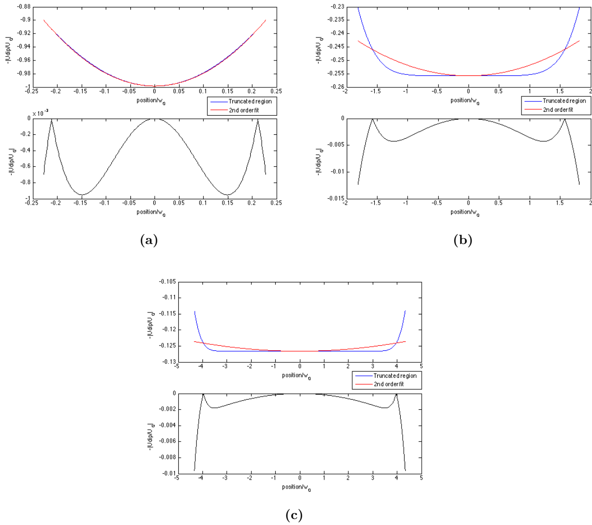
Figure 7.4: The top subplot shows the truncated distance corresponding to a tenth of the total trap depth (blue) and the second order polynomial fit to the dither range (red). A/w_0 values for (A)-(C) are 0.1, 4.9, and 9.9, respectively.
