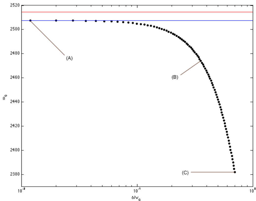
Figure 7.6: \omega_0 vs. \delta/w_0 where \delta is the distance over which the fit is performed, w_0 is the beam waist, \omega is the frequency over the corresponding distance of fitting \delta . The red line indicates the analytical value of \omega_0 and the blue line is the calculated value of \omega_0 . The fit range for which the variation from the calculated value of the maximum frequency lies within a percent is between 0.006 and 0.3.
