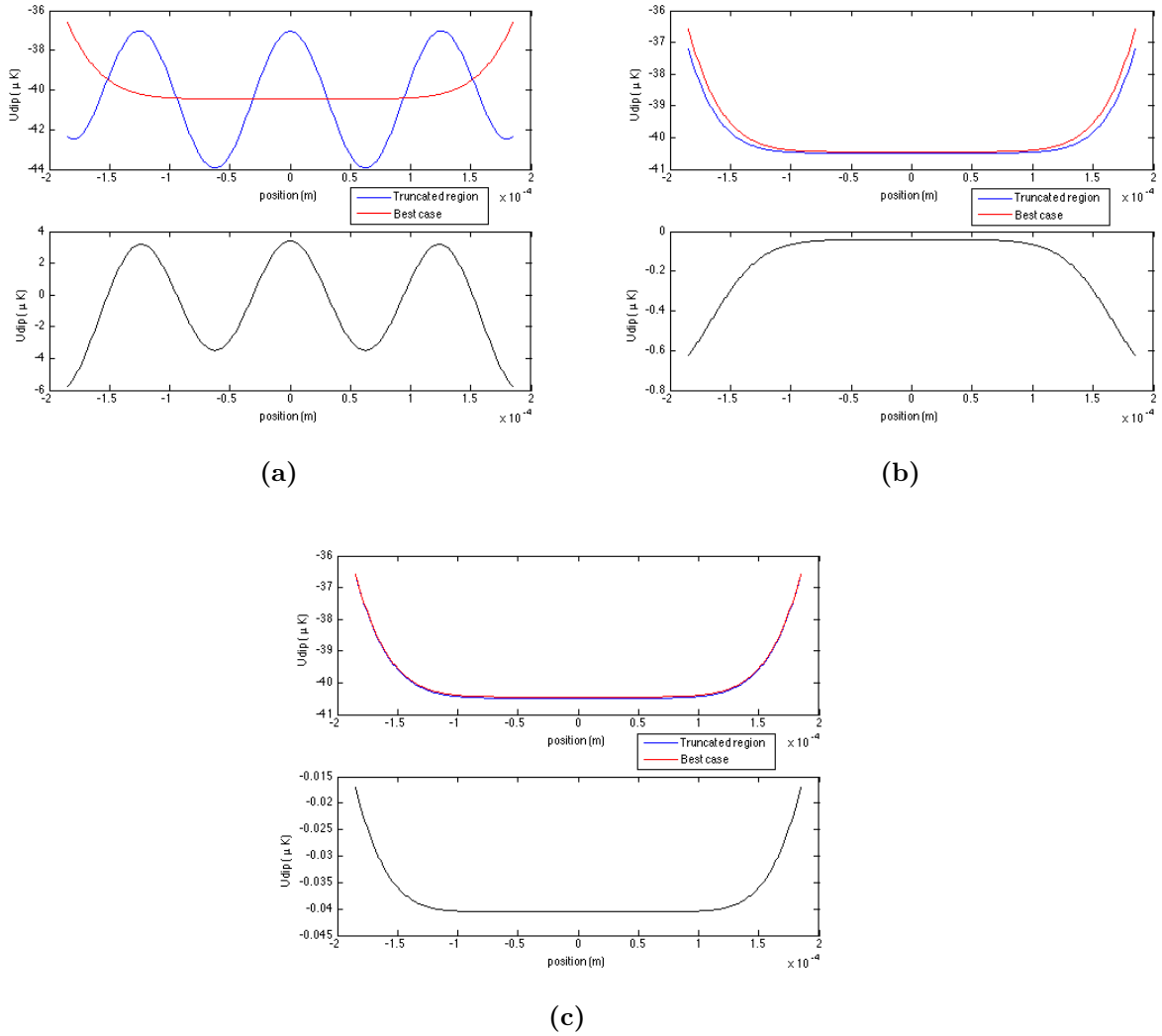
Figure 6.4: The top subplots (a)-(c) show the trapping potential of the truncated region (blue) and the best case potential having 1001 Gaussians (red). The bottom subplots show the residuals for each corresponding dither ranges having a s/w_0 value of (a) 1.25, (b) 0.63, and (c) 0.10. Note: (a)-(c) correspond to labels (A)-(C) in Figs. 6.2 and 6.3.
