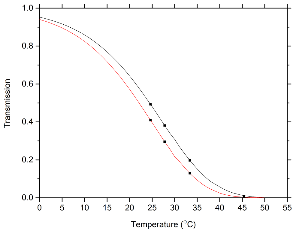
Figure 4.2: Transmission of the Doppler broadened Cs D2 line for different cell temperatures for the mixed species cell. All measurements were taken at zero detuning where maximum absorption is observed. The solid line shows the predicted transmission for a 1 cm pure cesium cell of the Doppler broadened F = 3 \rightarrow F = 2, 3, 4 (black) and F = 4 \rightarrow F = 3, 4, 5 (red) transitions.
