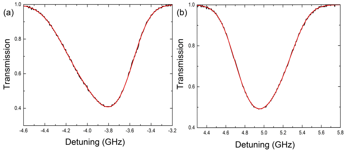
Figure 3.12: Doppler broadened transmission spectrum of the Cs D2 line for a 5 cm long, pure cesium cell, at a calculated temperature of 25°C. The black line shows the raw spectrum that has been adjacent averaged, and the red line is the temperature fit to the raw data performed by the algorithm. (a) shows the Doppler broadened spectrum for the F = 4 \rightarrow F' transitions and (b) for the F = 3 \rightarrow F' transitions of the 6^2S_{1/2} \rightarrow 6^2P_{3/2} energy levels
