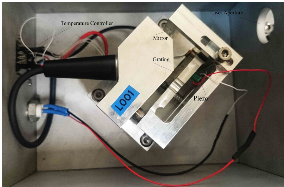
Figure 3.7: Home built 767 nm ECDL in Littrow configuration. The zeroth order beam is selected from the grating and outcoupled to the experiment.
