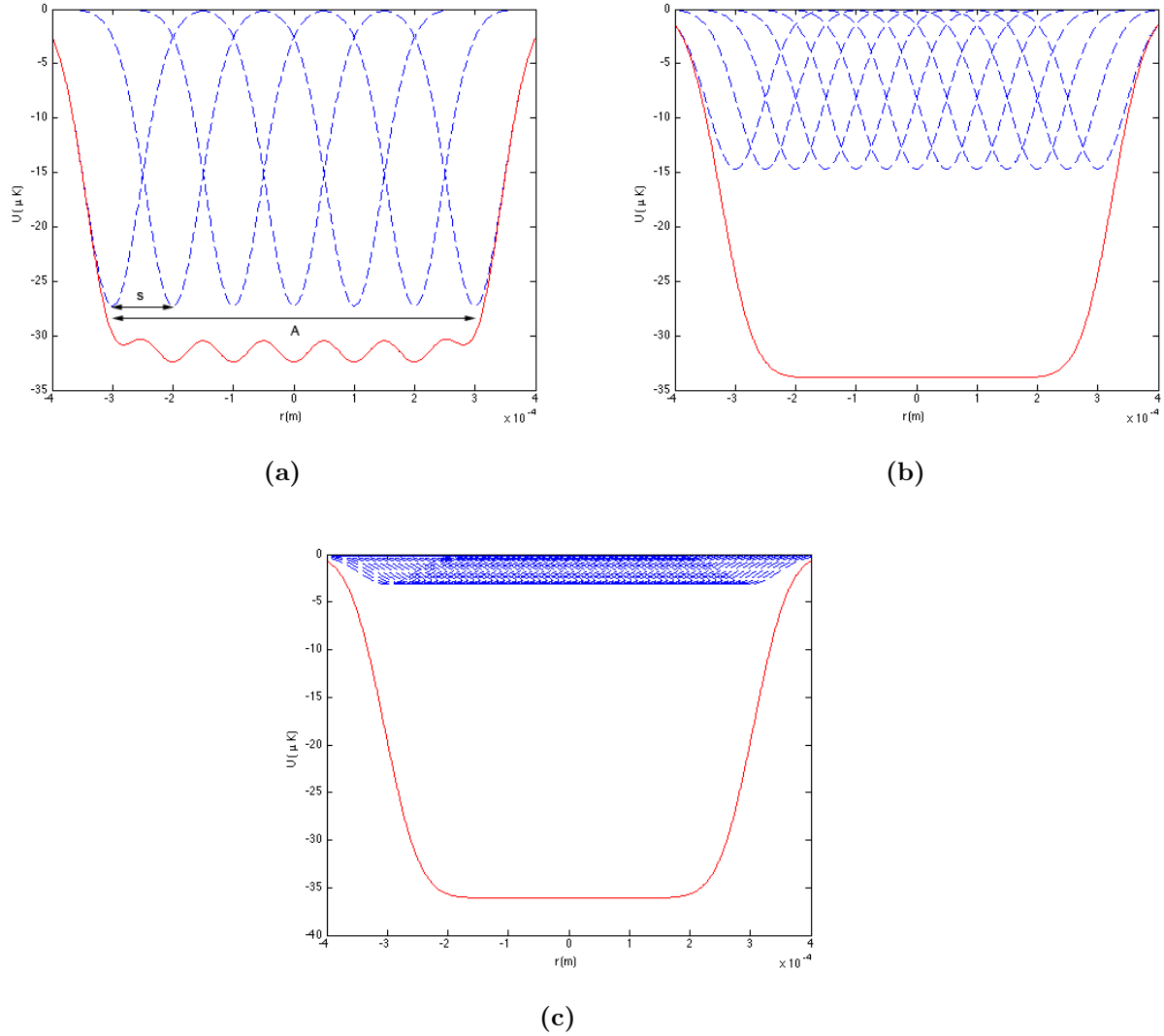
Figure 6.1: (a)-(c) shows the process of simulating a dithered Gaussian beam by superimposing multiple Gaussians, where adding a larger number of Gaussians result in a smoother summed potential. The summed potential is shown in red and the constituent Gaussians are shown in blue for (a) 7 constituent Gaussians, (b) 13 Gaussians and (c) 61 Gaussians. In the code, the summed potentials are normalised by dividing the calculated intensity by the number of Gaussians.
