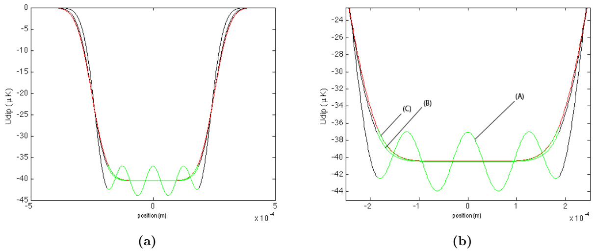
Figure 6.2: (a) Plot of dithered trapping potentials (black), best case potential containing 1001 Gaussians (red), and a tenth of the total trap depth of the dithered trapping potentials over which the RMS is calculated (green). (b) shows the same plot as (a) but over a smaller distance to distinguish the trapping potentials for different dither ranges. Labels (A)-(C) corresponds to dithered potentials with a s/w_0 value of (A) 1.25, (B) 0.625, and (C) 0.1.
