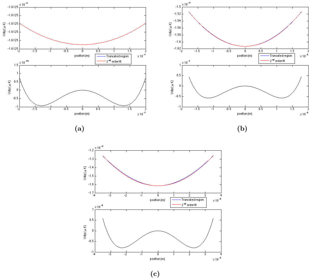
Figure 7.9: The top subplots (a)-(c) show the trapping potentials for different fit distances (blue) and the second order polynomial fits to the fit distances. Plots (a)-(c) correspond to (A)-(C) in Figs. 7.6 and 7.7. The fit distance as a fraction of the beam waist ( \delta/w_0 ) and the frequency calculation from the fits are (a) 0.004, 2.51 kHz (b) 0.36, 2.47 kHz and (c) 0.7, 2.38 kHz
