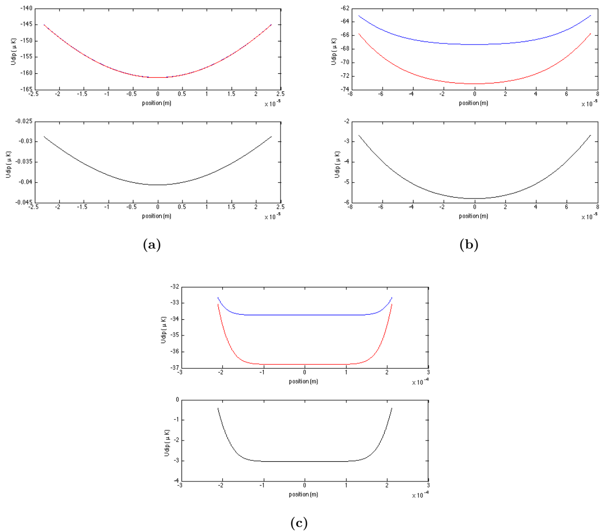
Figure 6.10: The top subplot of (a)-(c) show the trapping potential of the truncated region (blue) and the best case potential having 1101 Gaussians (red). The bottom subplot show the residuals corresponding to plots (A)-(C) in Fig. 6.8.
