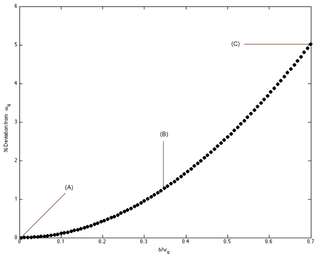
Figure 7.7: Percent deviation from the calculated value of \omega_0 vs. \delta/\omega_0 where \delta is the fitting distance which is proportional to the trap depth over which the fitting routine is performed and w_0 is the beam waist. The fit range for which the variation from the calculated value of the maximum frequency lies within a percent is between 0.006 and 0.3.
