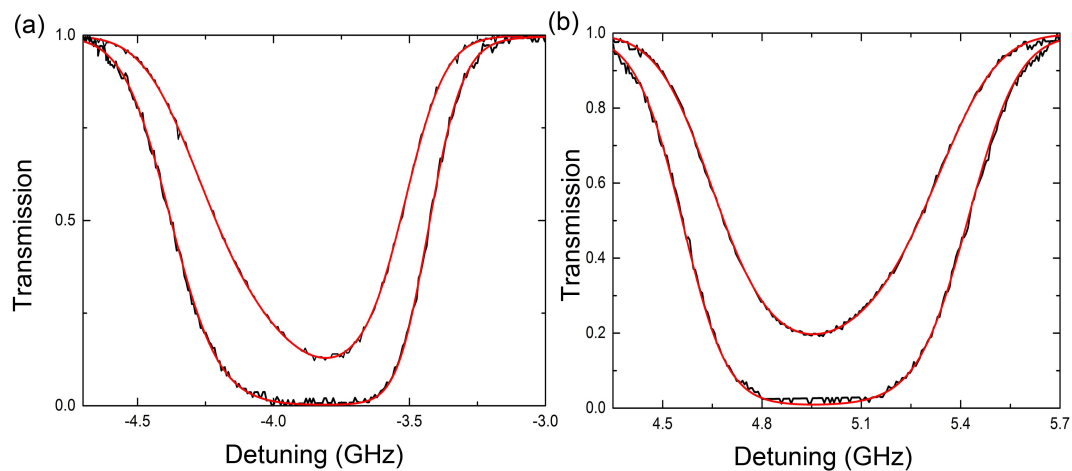
Figure 4.1: Doppler broadened transmission spectrum of the Cs D2 line for a mixed species at different temperatures. The black line shows the raw spectrum that has been smoothed, and the red line is the temperature fit to the raw data performed by the algorithm. The temperatures of the fitted curves are 24.6^{\circ}\text{C} and 45.4^{\circ}\text{C} for the shallower and deeper transmission spectrum, respectively. (a) and (b) show the transmission spectrum for the F = 4 line and F = 3 line, respectively.
