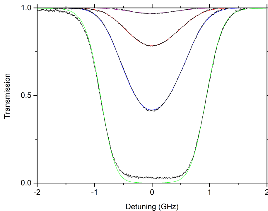
Figure 4.6: Overlay of the fitted transmission spectrum of the K D2 line for the mixture cell from Fig. 4.4. The black lines are the raw data and the temperatures resulting from the fitting routine are 32.8^\circ\text{C} (purple), 55.1^\circ\text{C} (red), 69.4^\circ\text{C} (blue), and 96.1^\circ\text{C} (green).
