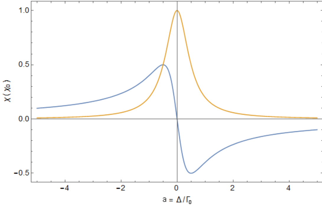
Figure 2.1: Plot of the real and imaginary components of susceptibility for a two-level system for an ensemble of atoms. The blue line indicates the real part and the orange line indicates the imaginary part.
