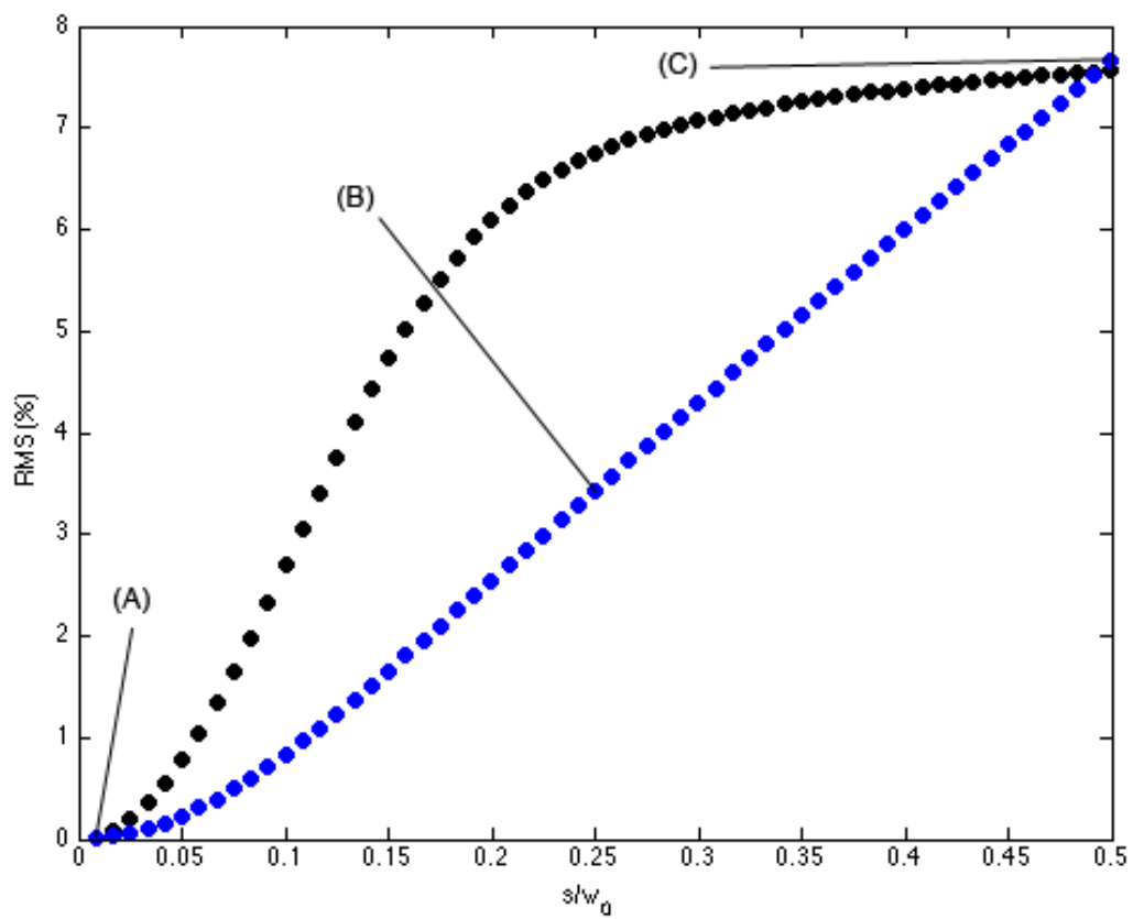
Figure 6.9: RMS across the entire pattern (black) and a tenth of the total trap depth (blue) of a dithered potential with the dither range set as a free parameter. Note: labels (A)-(C) correspond to plots (A)-(C) in Fig. 6.8.
