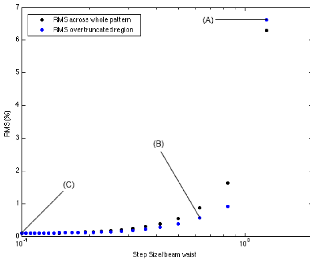
Figure 6.3: RMS across the entire pattern (black) and the truncated region corresponding to a tenth of the total trap depth (blue) of a dithered potential with the Gaussian number set as a free parameter between four Gaussians and 50 Gaussians in steps of two Gaussians, on a semi-logarithmic scale. Labels (A)-(C) corresponds to dithered potentials with a s/w_0 of (A) 1.25, (B) 0.625, and (C) 0.1, and also corresponds to the potential plots labeled in Fig. 6.2 (b)
