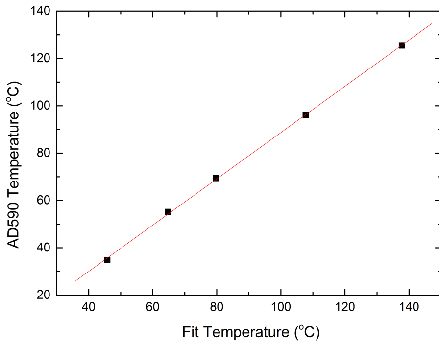
Figure 4.5: Comparison of the cell temperature measured using the AD590 transducer and the predicted cell temperature from Elecsus. The red line shows the linear fit to the raw data, where the slope from the fit is 1.0 \pm 0.1 and the intercept is 9 \pm 1 .
