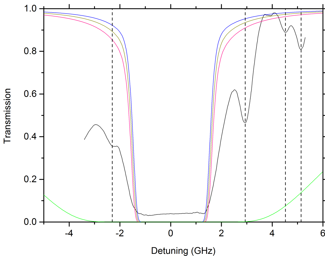
Figure 4.7: Transmission spectrum of the K D2 transition plotted against detuning at a cell temperature measured at 223 °C with a thermometer. The light green curve shows the calculated transmission profile at this temperature using a thermocouple. The cell temperature are approximated by overlaying prediction curves at 155 °C (blue), 165 °C (red), and 160 °C (dark green). The dashed lines indicate the absorption features observed at -2.3 GHz, 2.94 GHz, 4.52 GHz and 5.14 GHz.
