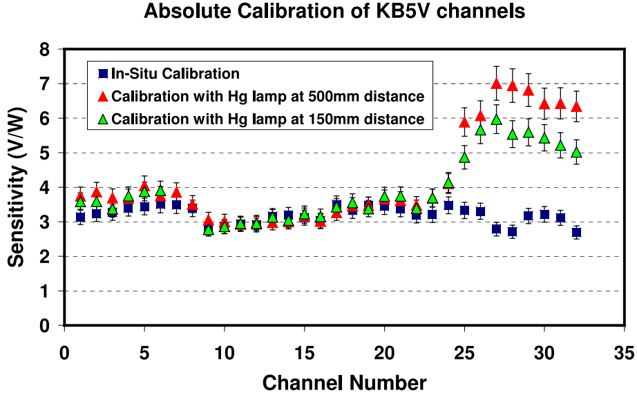
Figure 3.12: Comparison of in-situ electrical and mercury lamp measures of KB5 bolometer sensitivities. Although the two calibration methods agree well for channels 1 to 24, there is a discrepancy of roughly a factor of 2 between the methods for channels 25–32. These are the channels used by KB5F. Reproduced from [73]
