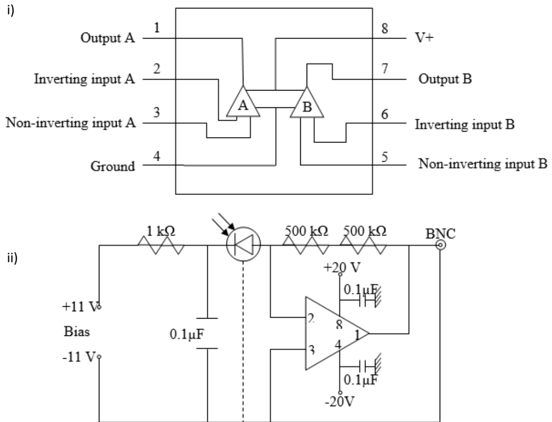
Figure 17: i) Schematic diagram of the NE5532P operational amplifier used in ii) The custom-built photodiode-based detector developed for HCARS. The initial resistor-capacitor combination acts a noise filter.
