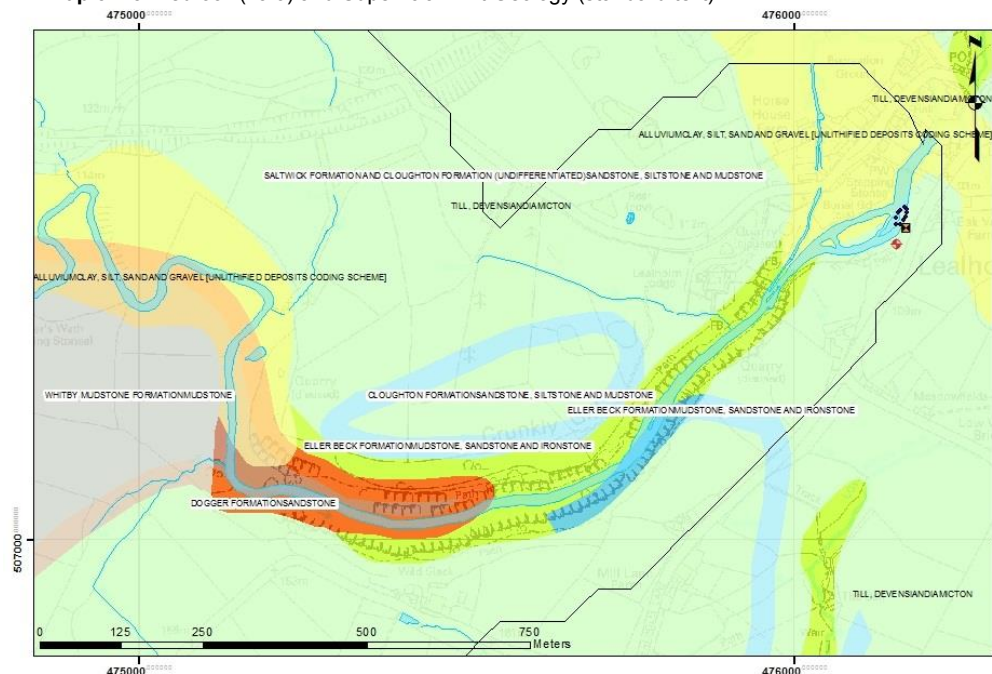
Map 3.7.3. Bedrock (halo) and Superficial Drift Geology (standard text)
