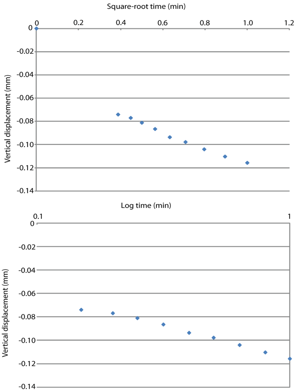
Figure 4.10 Time displacement curve of LA-11-GC5-1. 1 min loading of 3.7 kPa load.
