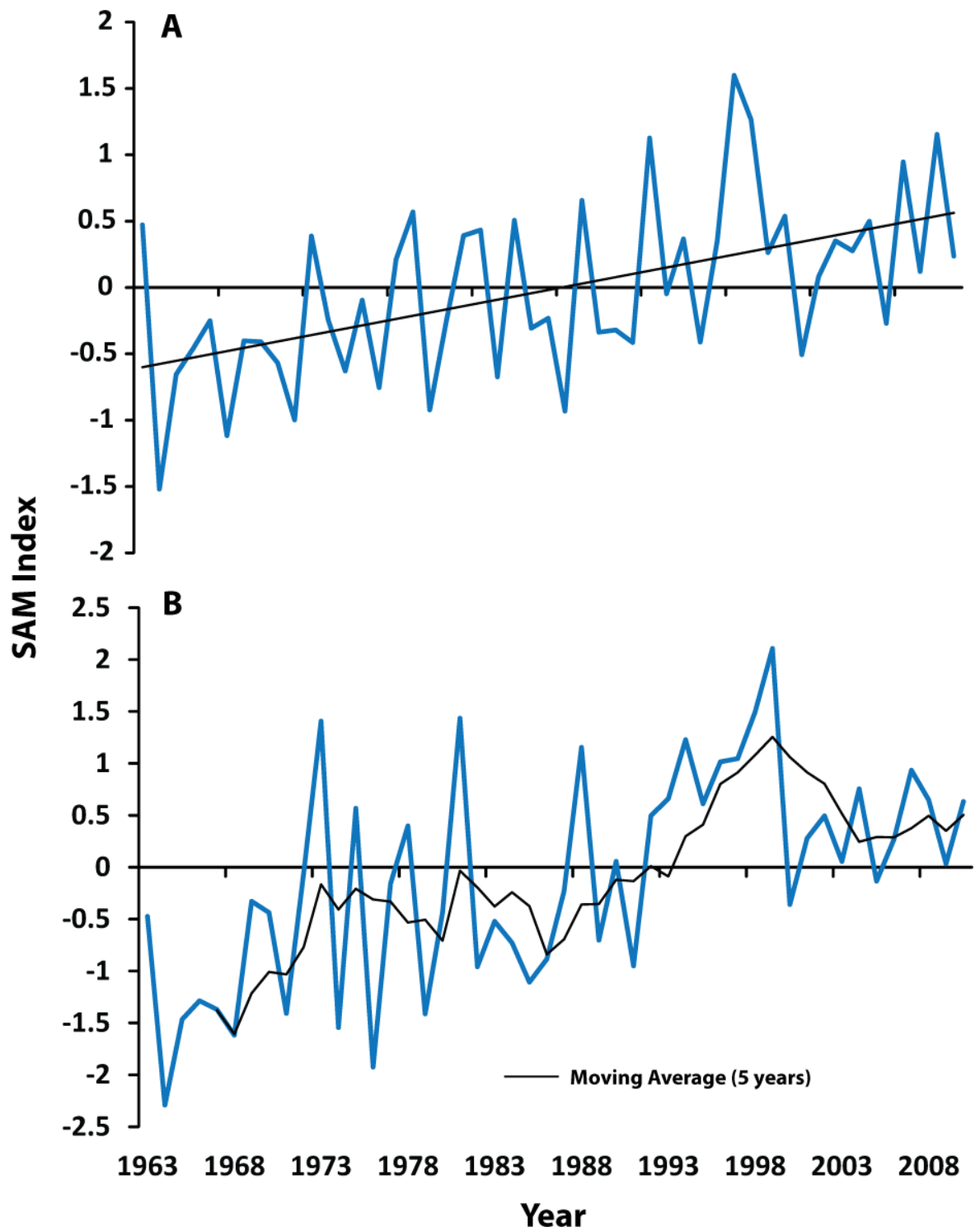
Figure 5.8: A) Annual averaged SAM index. B) December – May averaged SAM index. Data taken from http://www.nerc-bas.ac.uk/icd/gjma/sam.html (Marshall , 2003).
