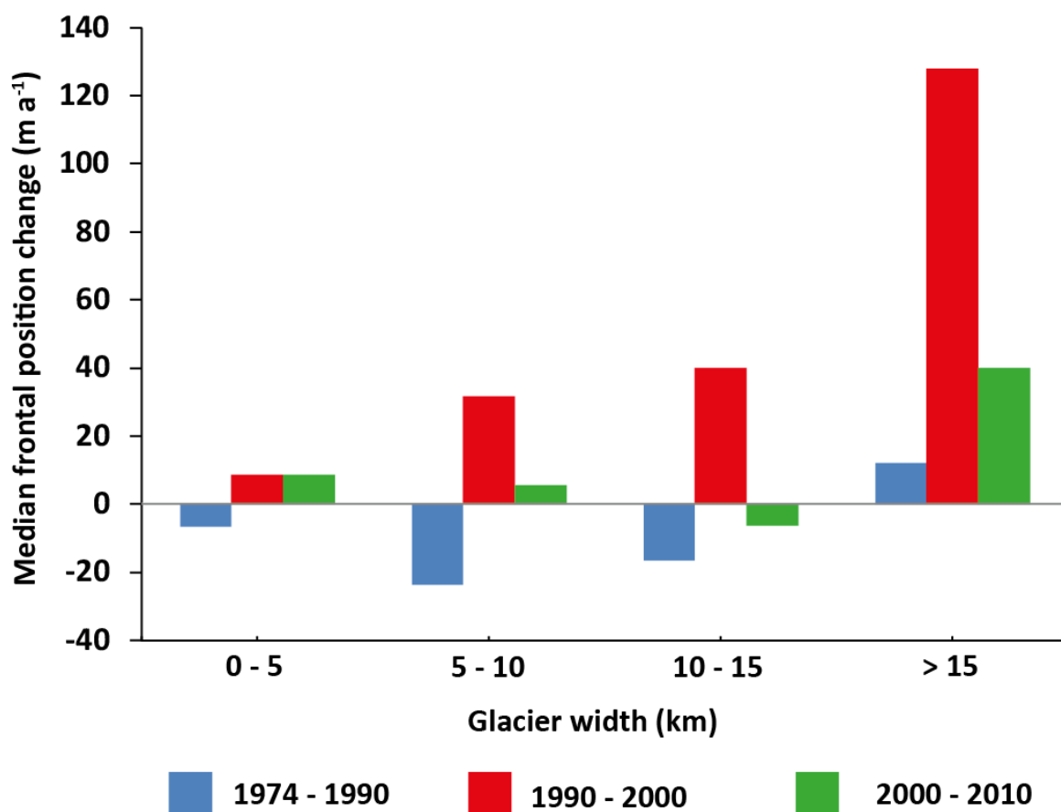
Figure 4.6: Median frontal position change for four glacier width classes, showing a general increase in magnitude in frontal position change as width increases and a consistent and robust trend showing the most negative frontal position change during the period 1974 to 1990 and the most positive between 1990 and 2000.
