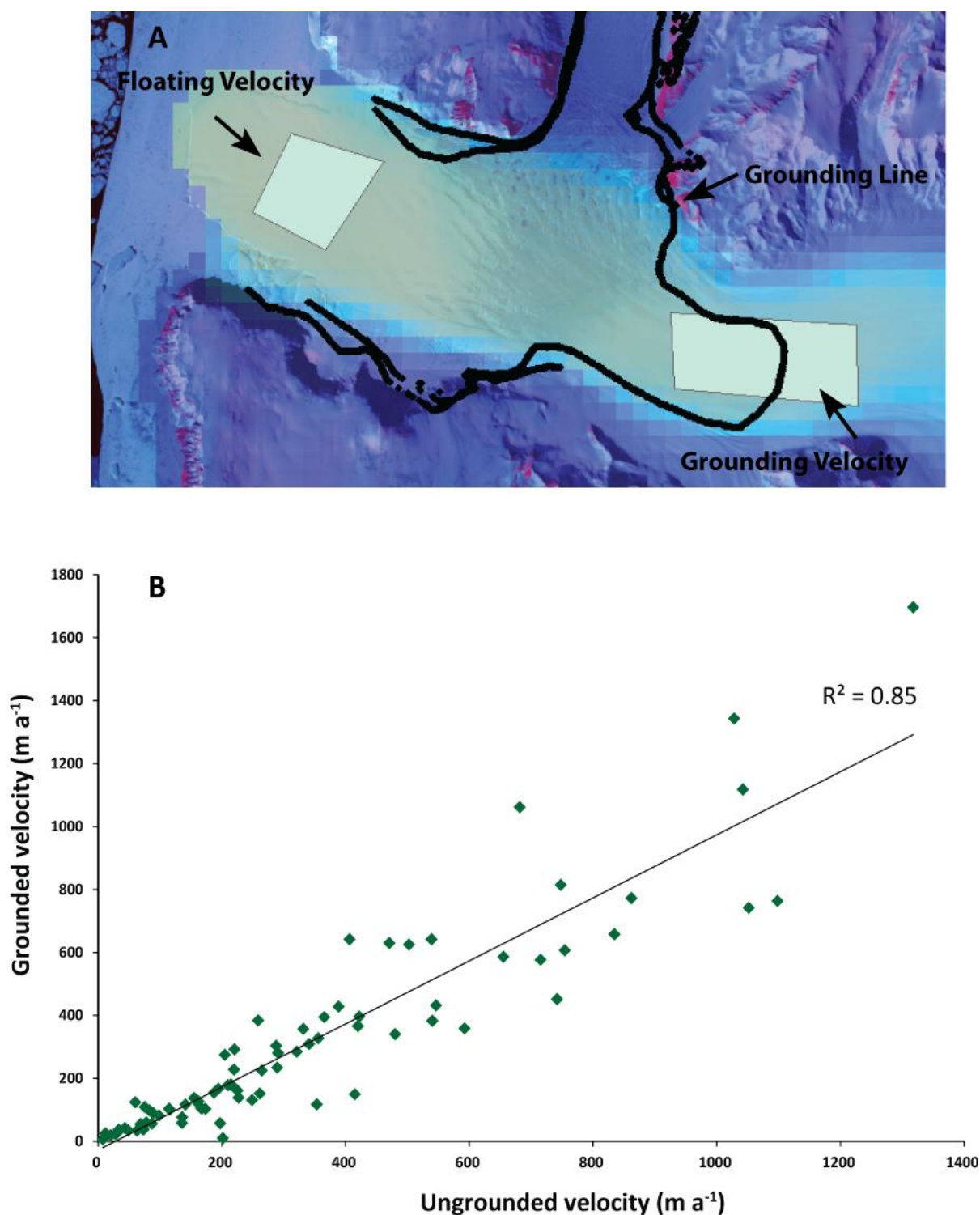
Figure 3.5: Extraction of flow speed data from Rignot (2011;b): a) Illustration showing where the grounding and floating velocity measurements were extracted. b) Scatter plot demonstrating the near linear relationship between flow speed extracted above and below the grounding line.
