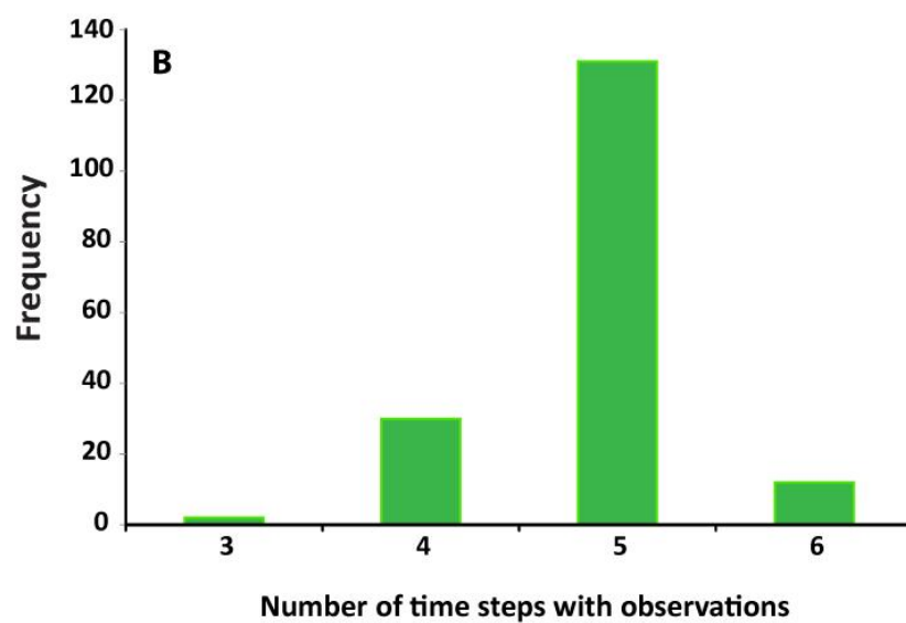
Figure 4.1 (A): Map showing the 175 glaciers mapped and which time steps they were mapped in. (B) Histogram showing how many time steps glaciers were mapped at each time step.
