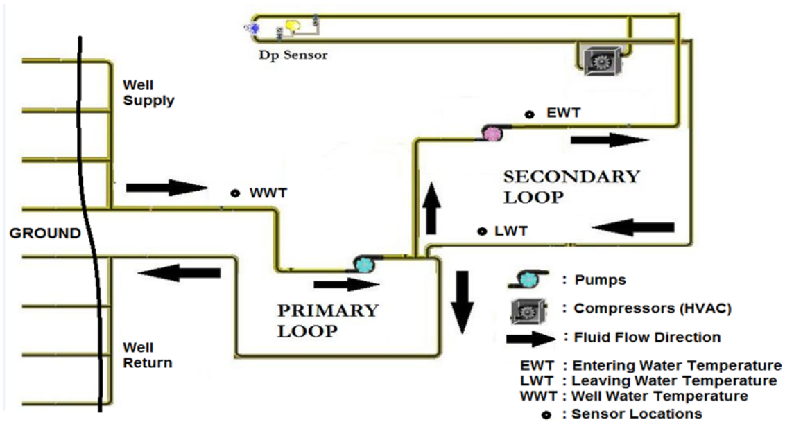
Figure 5.5: De-Coupled Primary-Secondary GSHP Loop Configuration
