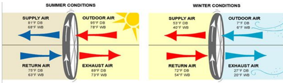
Figure 1.6: Example of ERV Operation
