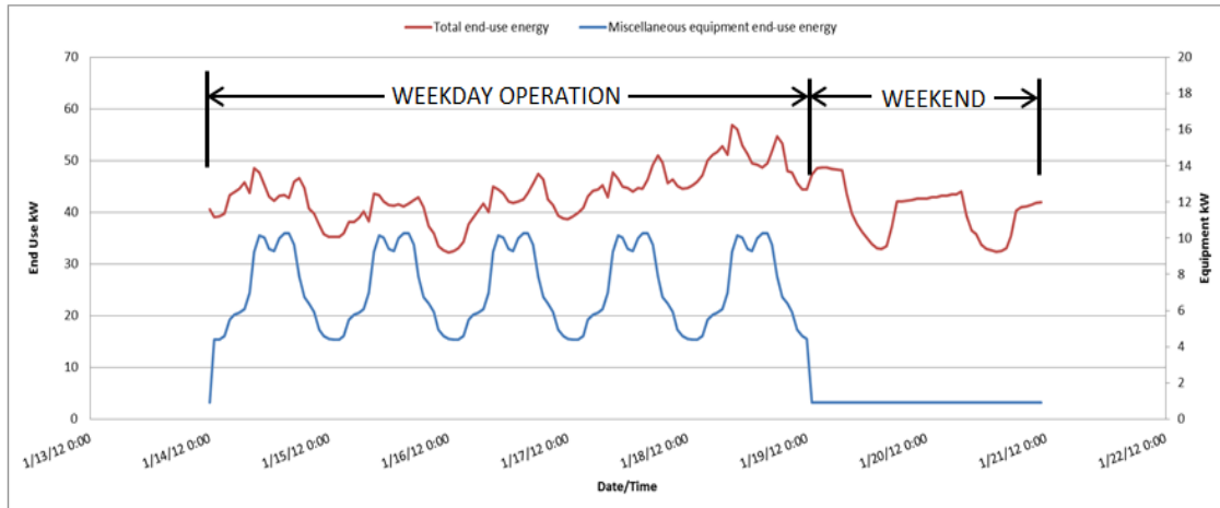
Figure 2.4: eQUEST Total Building Energy + Plug Load Consumption (1 Week)
