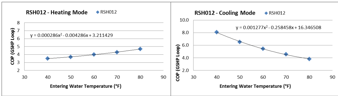
Figure 5.6: HP COP Performance Curves
