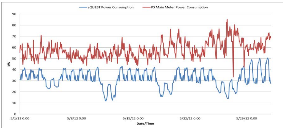
Figure 2.5: ESM Proposed Energy versus Actual Main Meter for 1 st Month
